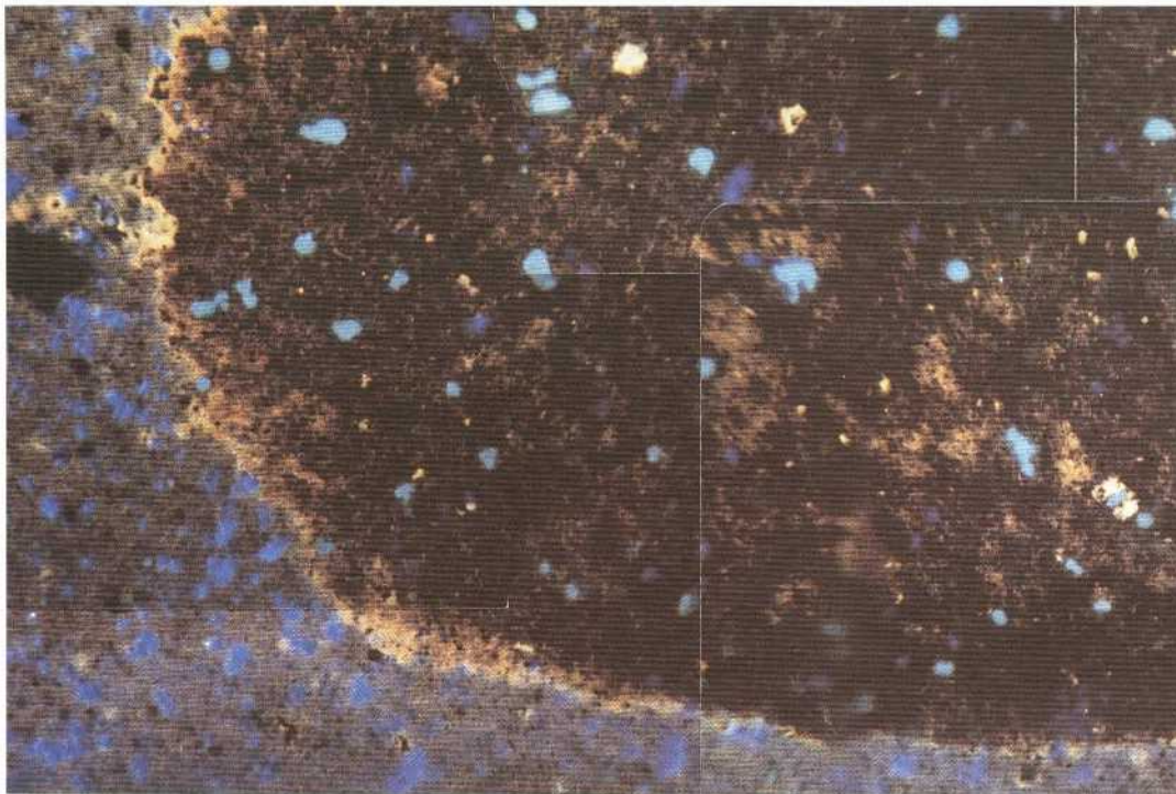
PLATE 6:1-8. Cathodoluminescence image of (two quarters of) a pitchblende nodule of total maximum diameter about 10 mm from a redox front in fine-grained phonolite. Note the non-emission of pitchblende impregnated (dark to black) portions of the nodule and the light yellowish-reddish emission of the illite – K-feldspar – kaolinite silicate mineral matrix of the nodule after pitchblende dissolution along the borders and in the left-hand part of the nodule (seen only in the upper photograph). Open pores in the nodule show light-blue or dark-(ink) blue emission (depending on the presence of preparation adhesives covering the glass support of the polished rock thin section) and dark- (ink) blue emission, if within the surrounding silicate matrix of the nodule (which was better impregnated by the preparation adhesives). The emission colours of the surrounding rock matrix are medium yellowish-grey and the finely disseminated black minerals are non-emitting (mostly submillimetric) pyrites. Compare with same nodule in plain light view (PLATE 6:1-9).
