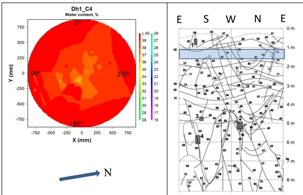
Figure 7-2. Left: Contour plot showing the water content distribution in block C4 in deposition hole 1. Right: Fracture mapping in deposition hole No 1. Water bearing fractures are marked with shaded areas, (Rhén and Forsmark 2001). The blue rectangle indicates the approximate position of block C4 relative to the fractures.
