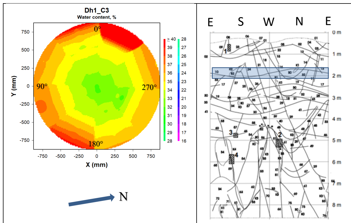
Figure 7-3. Left: Contour plot showing the water content distribution in block C3 in deposition hole 1. Right: Fracture mapping in deposition hole No 1. Water bearing fractures are marked with shaded areas, (Rhén and Forsmark 2001). The blue rectangle indicates the approximate position of block C3 relative to the fractures.
