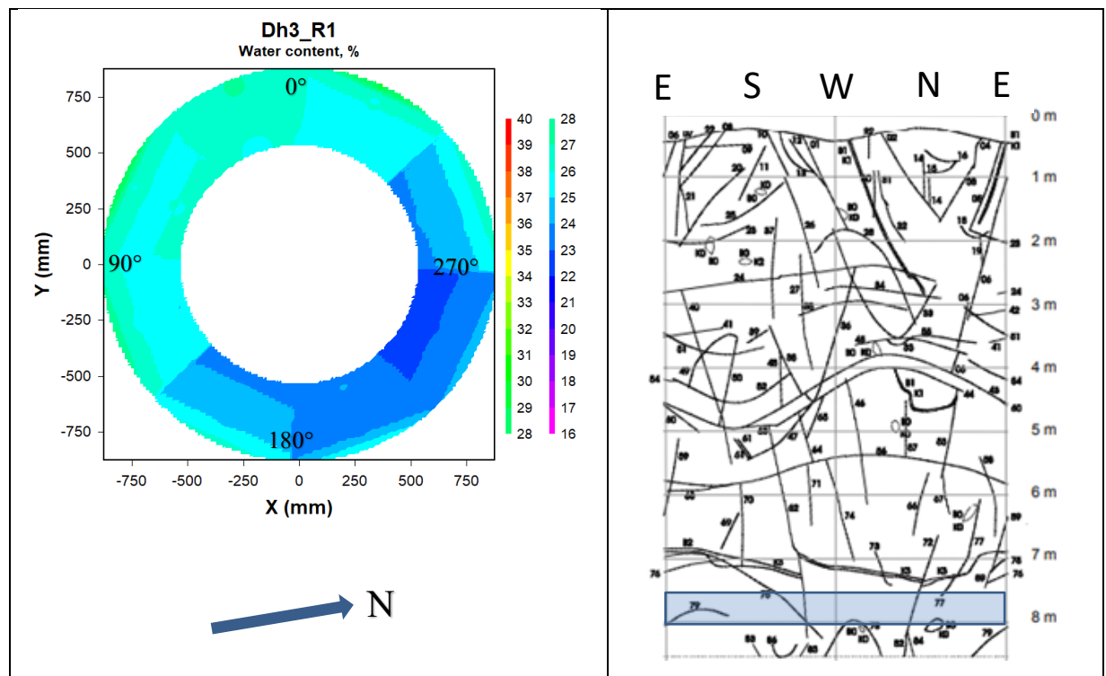
Figure 5-14. Left: Contour plot showing the water content distribution in block R1 in deposition hole 3. Right: Fracture mapping in deposition hole No 3. Water bearing fractures are marked with shaded areas (no such areas in this deposition hole), (Rhén and Forsmark 2001). The blue rectangle indicates the approximate position of block R1 relative to the fractures.
