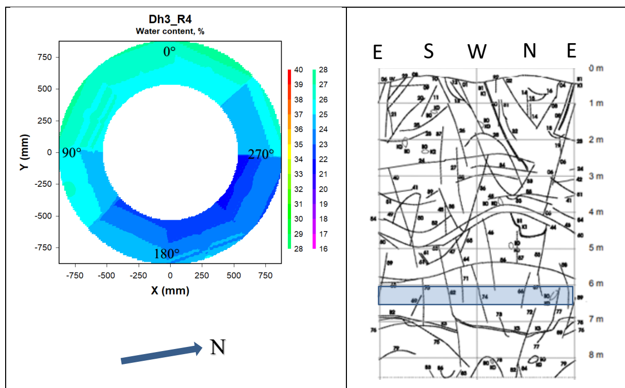
Figure 5-11. Left: Contour plot showing the water content distribution in block R4 in deposition hole 3. Right: Fracture mapping in deposition hole No 3. Water bearing fractures are marked with shaded areas (no such areas in this deposition hole), (Rhén and Forsmark 2001). The blue rectangle indicates the approximate position of block R4 relative to the fractures.
