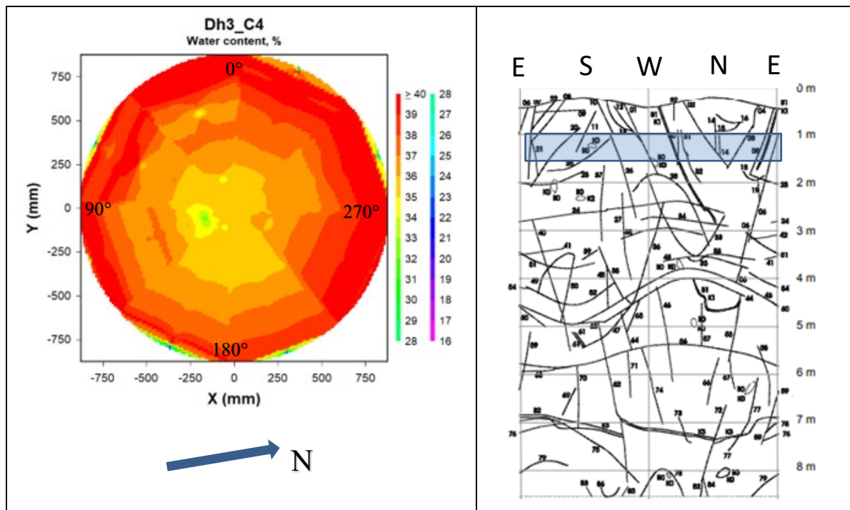
Figure 5-2. Left: Contour plot showing the water content distribution in block C4 in deposition hole 3. Right: Fracture mapping in deposition hole No 3. Water bearing fractures are marked with shaded areas (no such areas in this deposition hole), (Rhén and Forsmark 2001). The blue rectangle indicates the approximate position of block C4 relative to the fractures.
