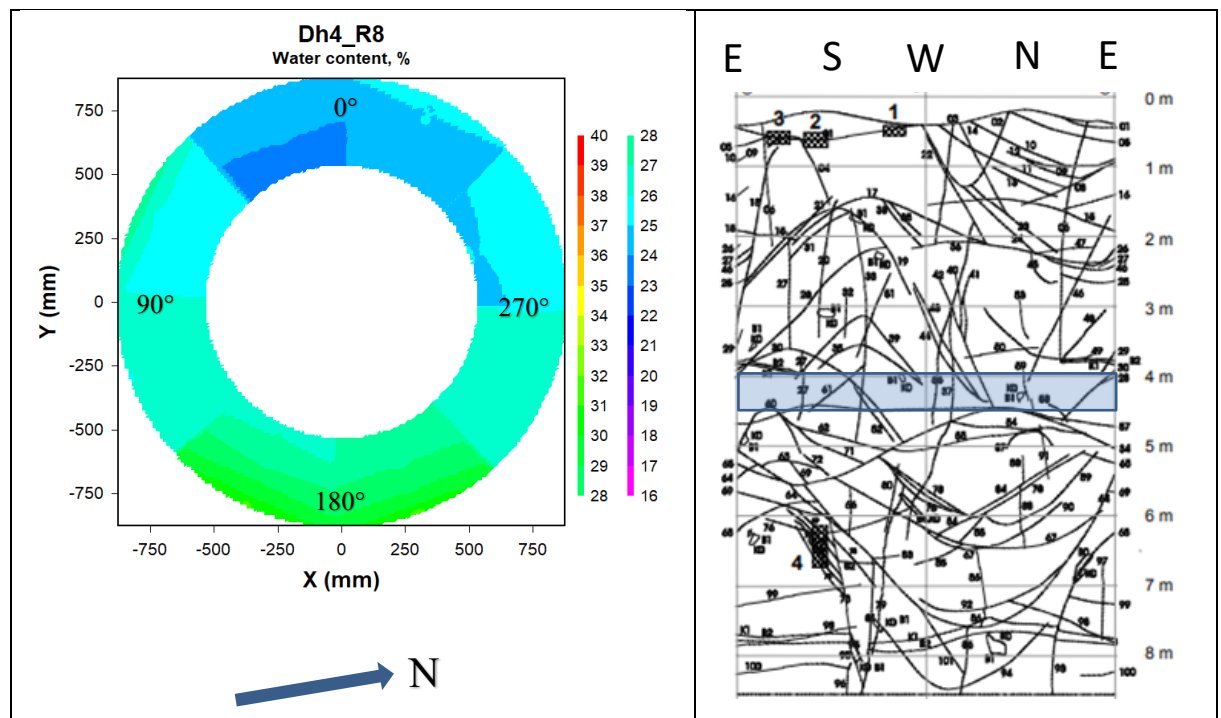
Figure 4-7. Left: Contour plot showing the water content distribution in block R8 in deposition hole 4. The degrees given are those used for sampling. Right: Fracture mapping in deposition hole No 4. Water bearing fractures are marked with shaded areas, (Rhén and Forsmark 2001). The blue rectangle indicates the approximate position of block R8 relative to the fractures.
