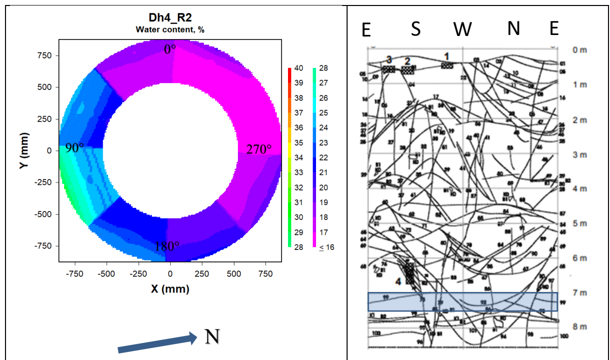
Figure 4-13. Left: Contour plot showing the water content distribution in block R2 in deposition hole 4. The degrees given are those used for sampling. Right: Fracture mapping in deposition hole No 4. Water bearing fractures are marked with shaded areas, (Rhén and Forsmark 2001). The blue rectangle indicates the approximate position of block R2 relative to the fractures.
