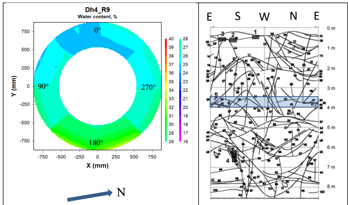
Figure 4-6. Left: Contour plot showing the water content distribution in block R9 in deposition hole 4. The degrees given are those used for sampling. Right: Fracture mapping in deposition hole No 4. Water bearing fractures are marked with shaded areas, (Rhén and Forsmark 2001). The blue rectangle indicates the approximate position of block R9 relative to the fractures.
