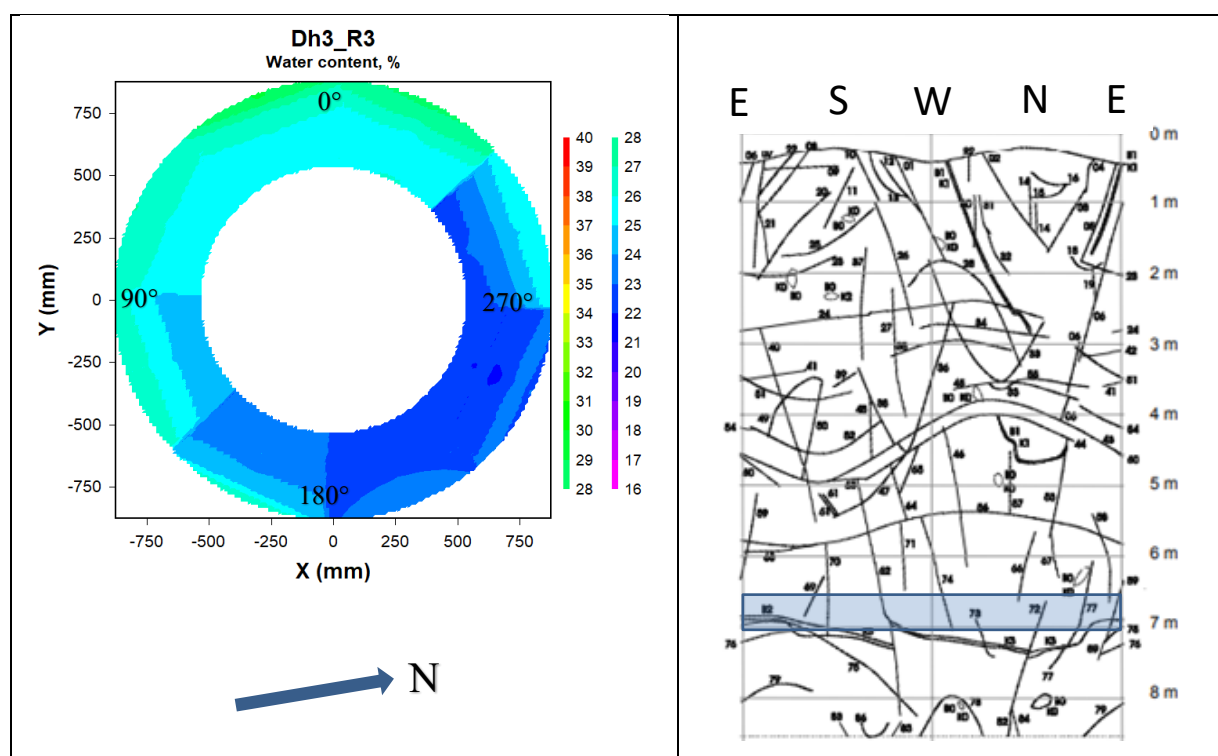
Figure 5-12. Left: Contour plot showing the water content distribution in block R3 in deposition hole 3. Right: Fracture mapping in deposition hole No 3. Water bearing fractures are marked with shaded areas (no such areas in this deposition hole), (Rhén and Forsmark 2001). The blue rectangle indicates the approximate position of block R3 relative to the fractures.
