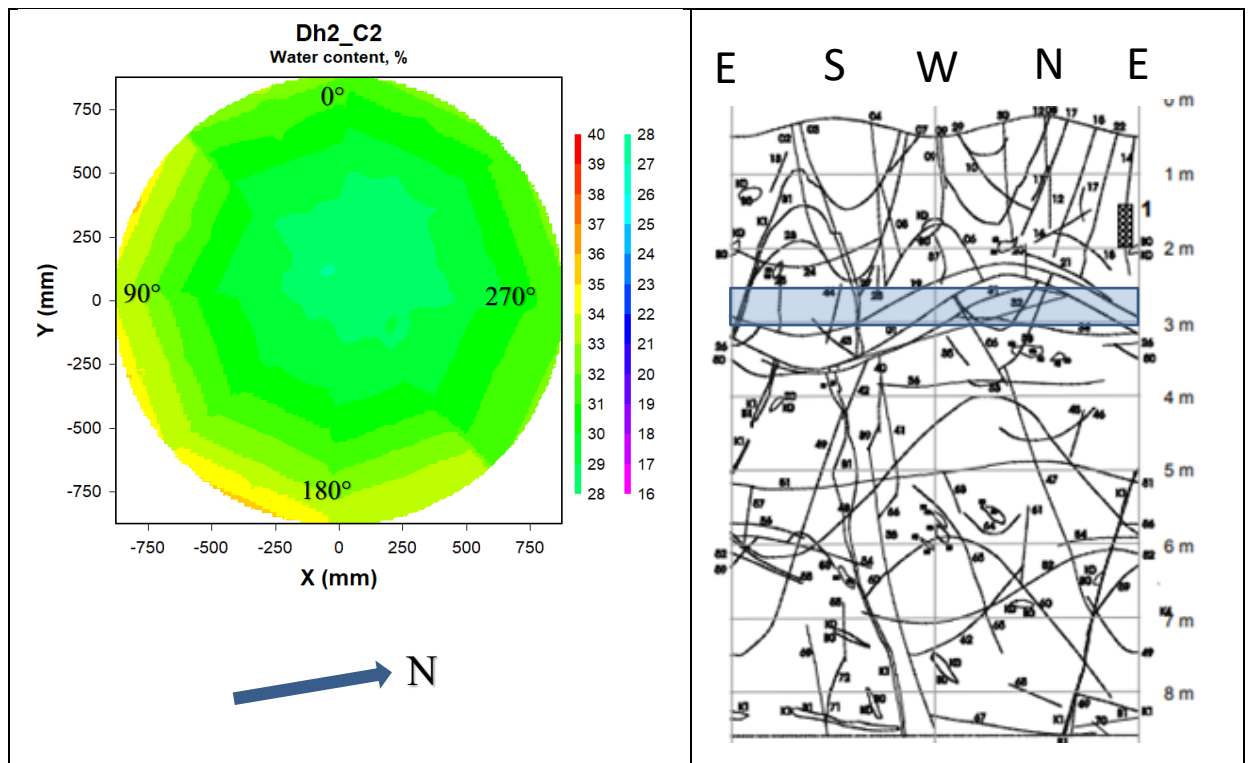
Figure 6-4. Left: Contour plot showing the water content distribution in block C2 in deposition hole 2. Right: Fracture mapping in deposition hole No 2. Water bearing fractures are marked with shaded areas, (Rhén and Forsmark 2001). The blue rectangle indicates the approximate position of block C2 relative to the fractures.
