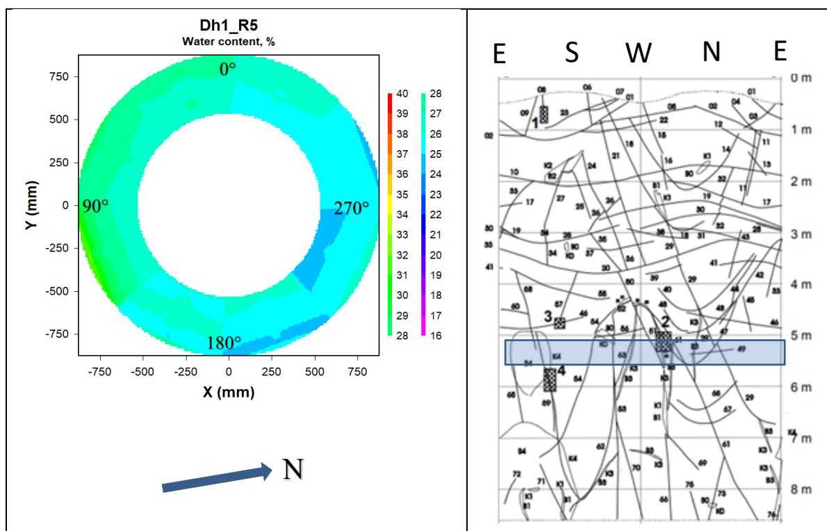
Figure 7-10. Left: Contour plot showing the water content distribution in block R5 in deposition hole 1. Right: Fracture mapping in deposition hole No 1. Water bearing fractures are marked with shaded areas, (Rhén and Forsmark 2001). The blue rectangle indicates the approximate position of block R5 relative to the fractures.
