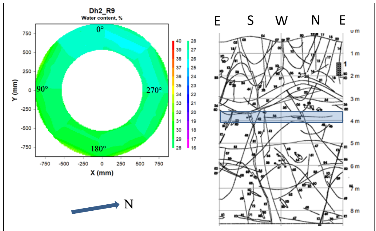
Figure 6-6. Left: Contour plot showing the water content distribution in block R9 in deposition hole 2. Right: Fracture mapping in deposition hole No 2. Water bearing fractures are marked with shaded areas (no such areas in this deposition hole), (Rhén and Forsmark 2001). The blue rectangle indicates the approximate position of block R9 relative to the fractures.
