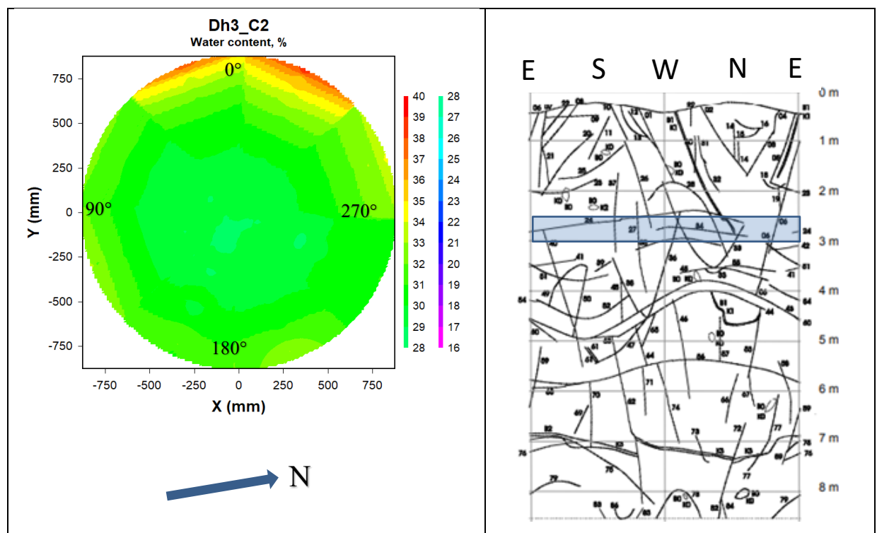
Figure 5-4. Left: Contour plot showing the water content distribution in block C2 in deposition hole 3. Right: Fracture mapping in deposition hole No 3. Water bearing fractures are marked with shaded areas (no such areas in this deposition hole), (Rhén and Forsmark 2001). The blue rectangle indicates the approximate position of block C2 relative to the fractures.
