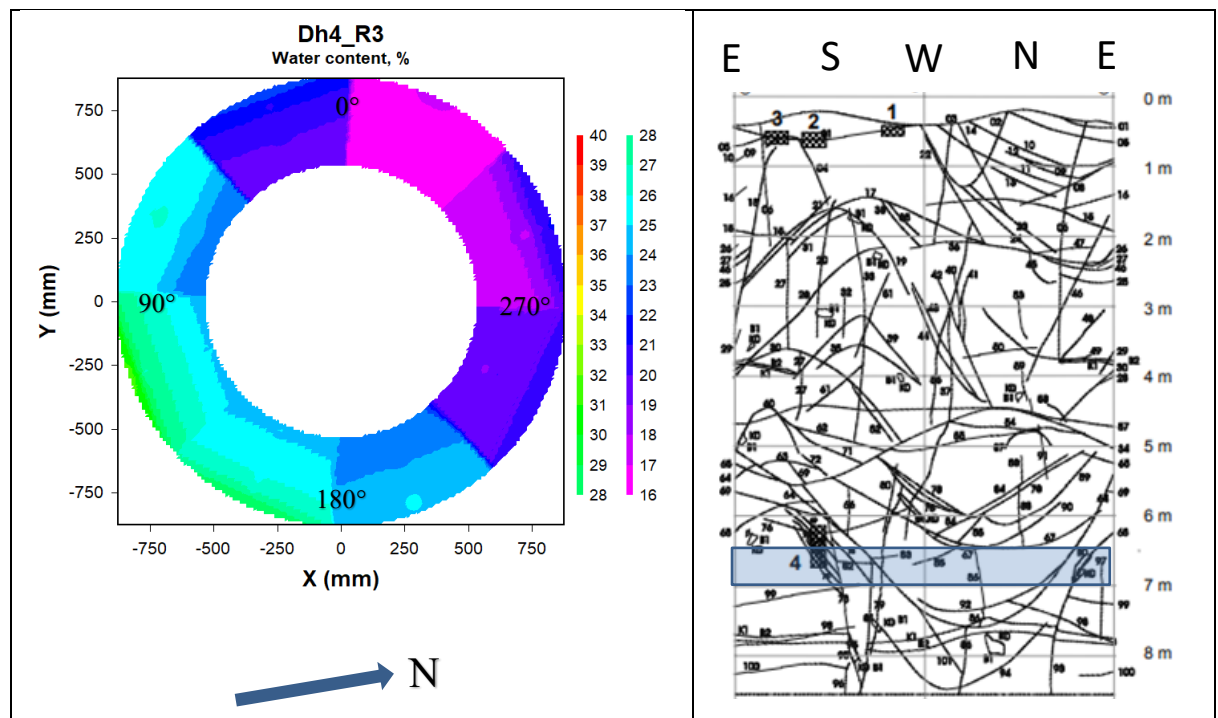
Figure 4-12. Left: Contour plot showing the water content distribution in block R3 in deposition hole 4. The degrees given are those used for sampling. Right: Fracture mapping in deposition hole No 4. Water bearing fractures are marked with shaded areas, (Rhén and Forsmark 2001). The blue rectangle indicates the approximate position of block R3 relative to the fractures.
