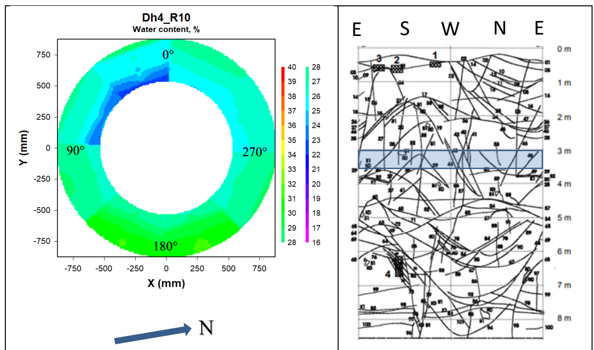
Figure 4-5. Left: Contour plot showing the water content distribution in block R10 in deposition hole 4. The degrees given are those used for sampling. Right: Fracture mapping in deposition hole No 4. Water bearing fractures are marked with shaded areas, (Rhén and Forsmark 2001). The blue rectangle indicates the approximate position of block R10 relative to the fractures.
