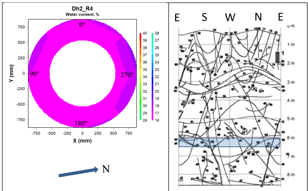
Figure 6-11. Left: Contour plot showing the water content distribution in block R4 in deposition hole 2. Right: Fracture mapping in deposition hole No 2. Water bearing fractures are marked with shaded areas (no such areas in this deposition hole), (Rhén and Forsmark 2001). The blue rectangle indicates the approximate position of block R4 relative to the fractures.
