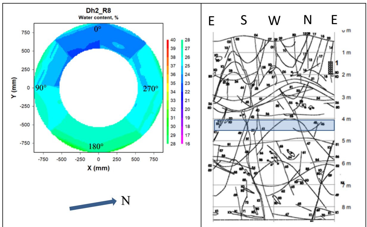
Figure 6-7. Left: Contour plot showing the water content distribution in block R8 in deposition hole 2. Right: Fracture mapping in deposition hole No 2. Water bearing fractures are marked with shaded areas (no such areas in this deposition hole), (Rhén and Forsmark 2001). The blue rectangle indicates the approximate position of block R8 relative to the fractures.
