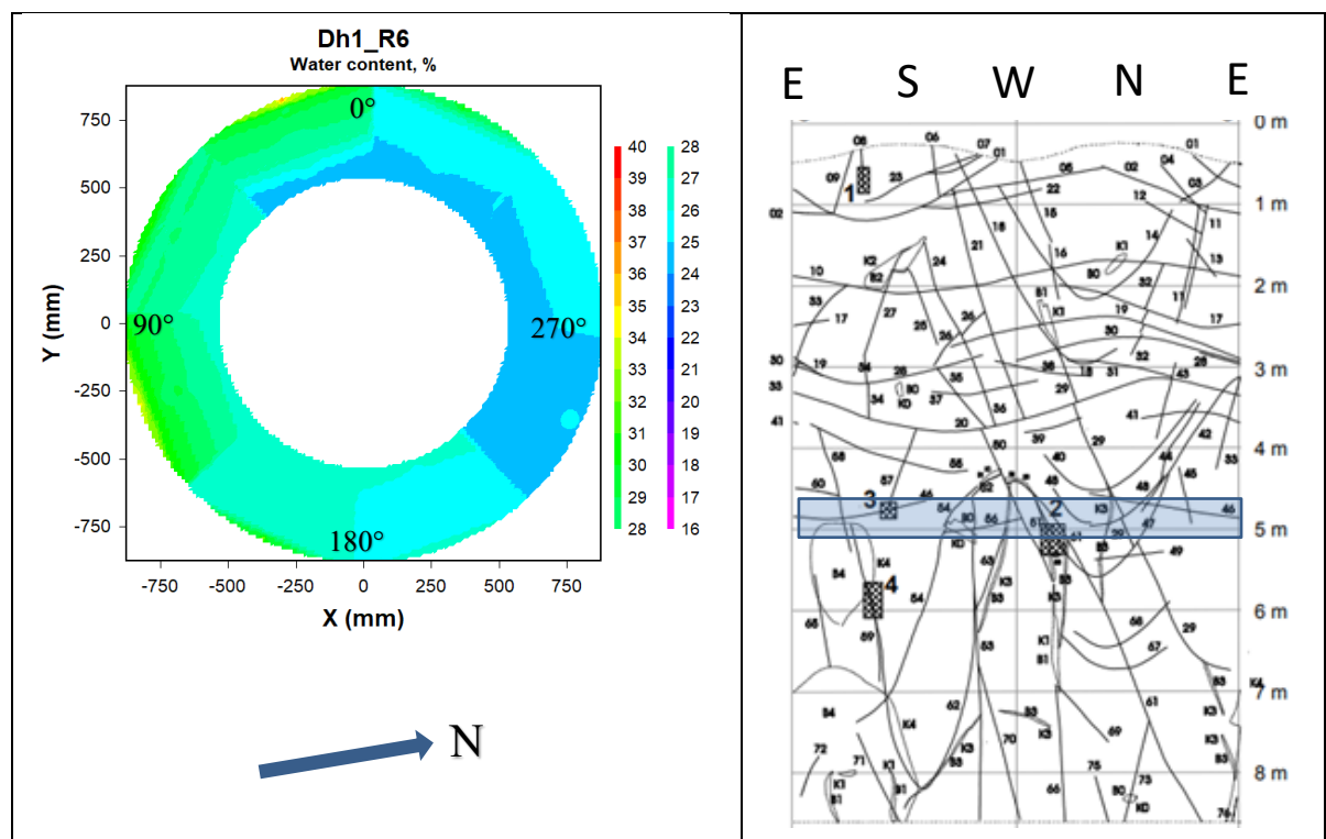
Figure 7-9. Left: Contour plot showing the water content distribution in block R6 in deposition hole 1. Right: Fracture mapping in deposition hole No 1. Water bearing fractures are marked with shaded areas, (Rhén and Forsmark 2001). The blue rectangle indicates the approximate position of block R6 relative to the fractures.
