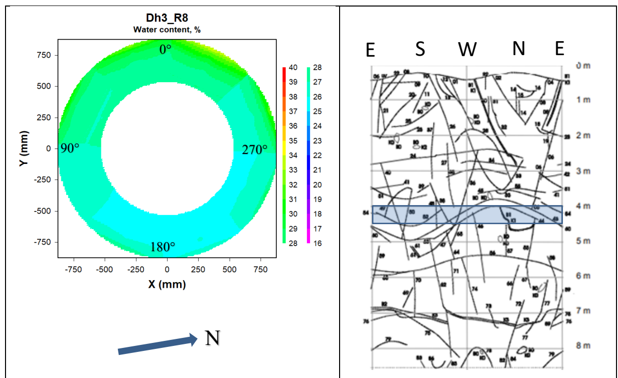
Figure 5-7. Left: Contour plot showing the water content distribution in block R8 in deposition hole 3. Right: Fracture mapping in deposition hole No 3. Water bearing fractures are marked with shaded areas (no such areas in this deposition hole), (Rhén and Forsmark 2001). The blue rectangle indicates the approximate position of block R8 relative to the fractures.
