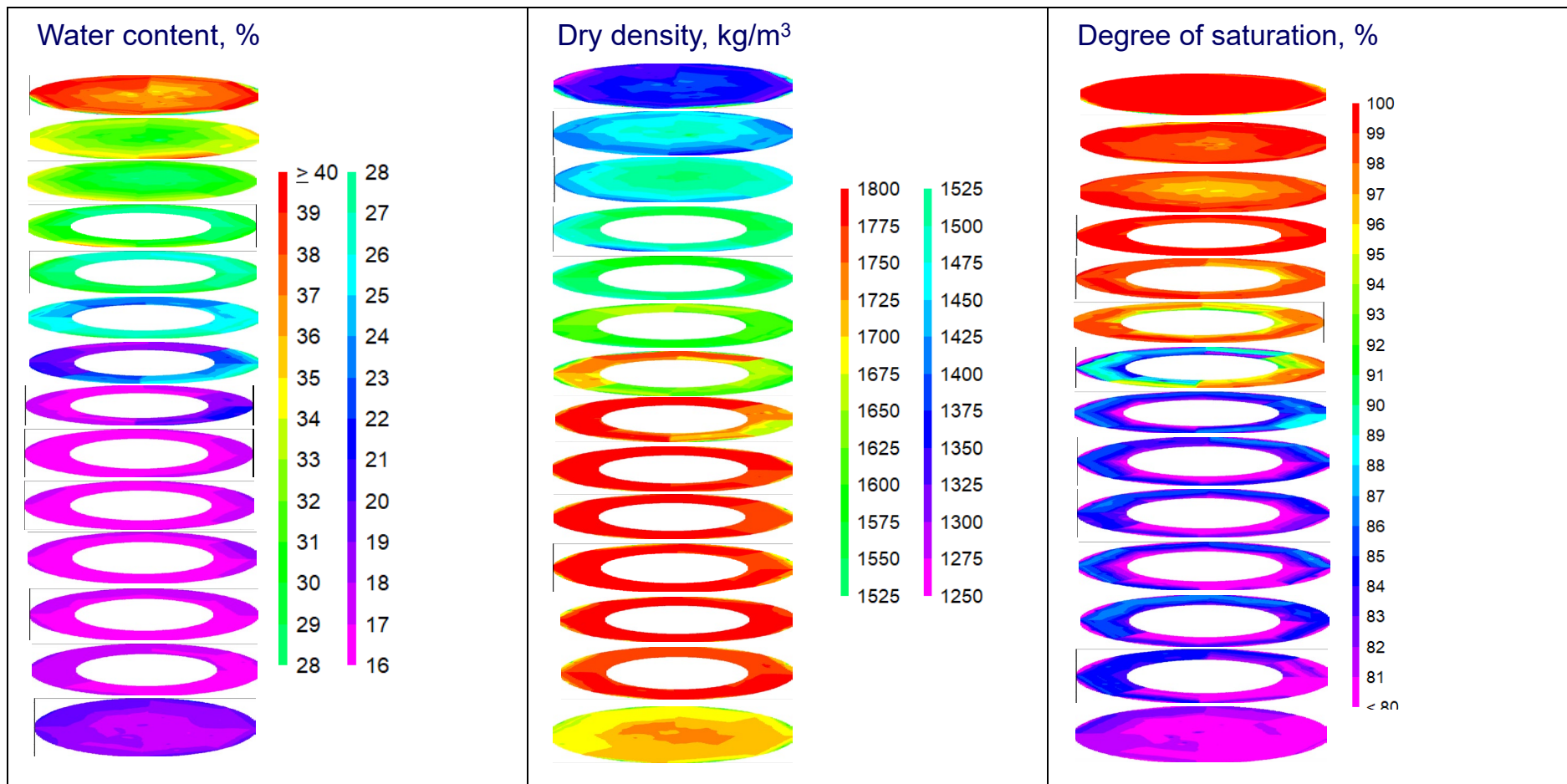
Figure 6-16. Compressed contour plots of every single block in Dh 2 stacked on each other. Left: the water content distribution (%) Middle: the dry density distribution ( \text{kg/m}^3 ) Right: the degree of saturation distribution (%).
