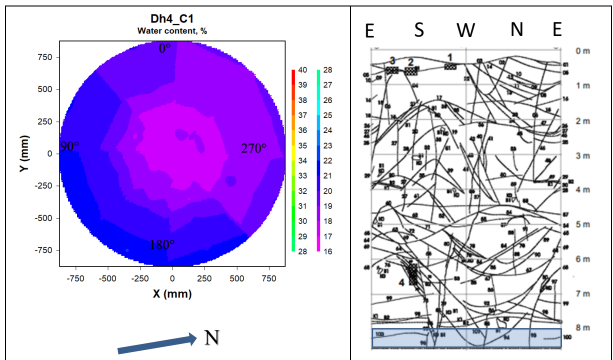
Figure 4-15. Left: Contour plot showing the water content distribution in block C1 in deposition hole 4. The degrees given are those used for sampling. Right: Fracture mapping in deposition hole No 4. Water bearing fractures are marked with shaded areas, (Rhén and Forsmark 2001). The blue rectangle indicates the approximate position of block C1 relative to the fractures.
