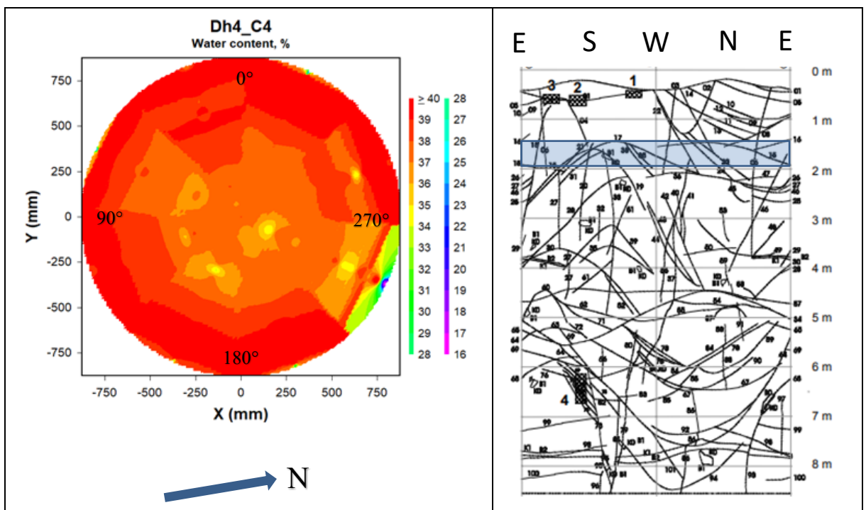
Figure 4-2. Left: Contour plot showing the water content distribution in block C4 in deposition hole 4. The degrees given are those used for sampling. Right: Fracture mapping in deposition hole No 4. Water bearing fractures are marked with shaded areas, (Rhén and Forsmark 2001). The blue rectangle indicates the approximate position of block C4 relative to the fractures.
