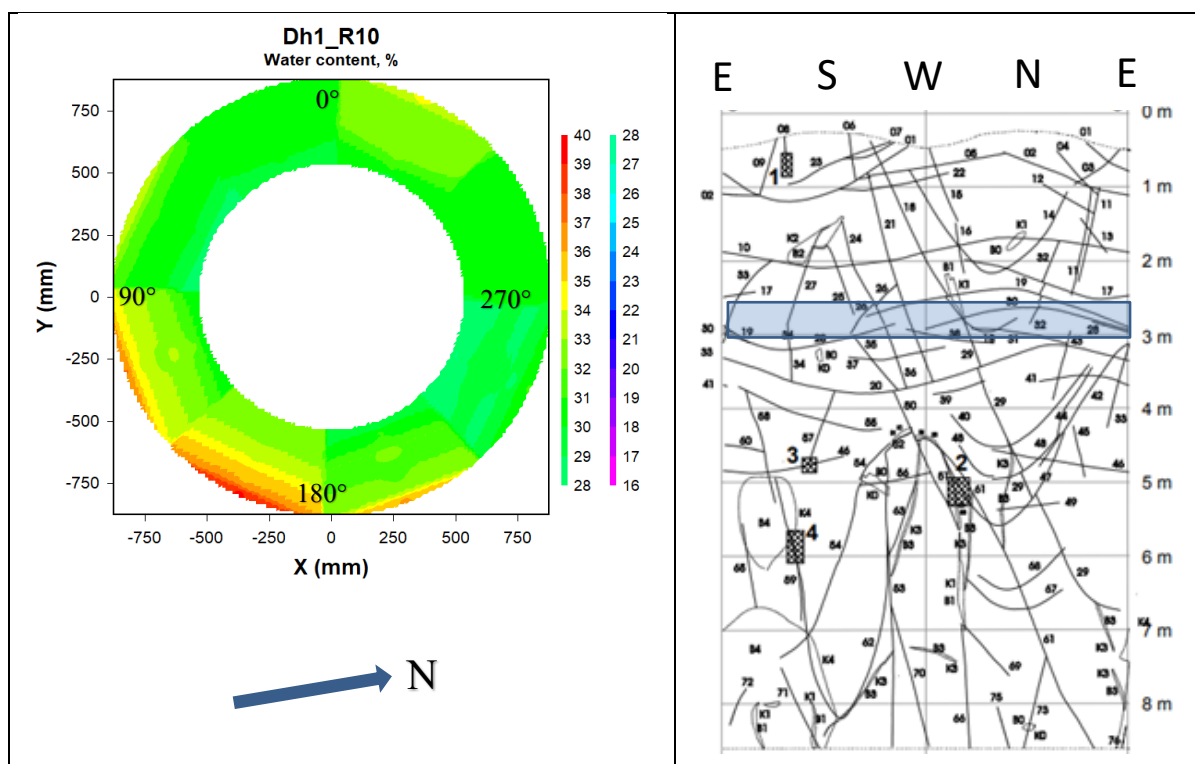
Figure 7-5. Left: Contour plot showing the water content distribution in block R10 in deposition hole 1. Right: Fracture mapping in deposition hole No 1. Water bearing fractures are marked with shaded areas, (Rhén and Forsmark 2001). The blue rectangle indicates the approximate position of block R10 relative to the fractures.
