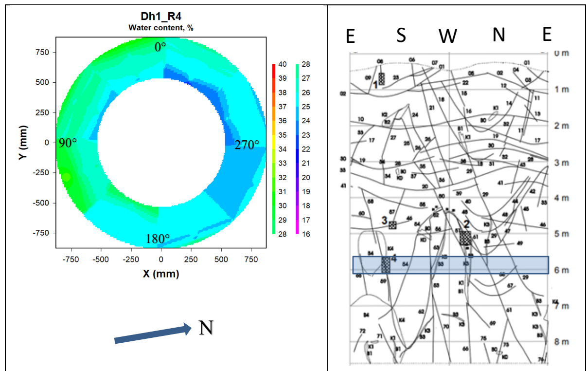
Figure 7-11. Left: Contour plot showing the water content distribution in block R4 in deposition hole 1. Right: Fracture mapping in deposition hole No 1. Water bearing fractures are marked with shaded areas, (Rhén and Forsmark 2001). The blue rectangle indicates the approximate position of block R4 relative to the fractures.
