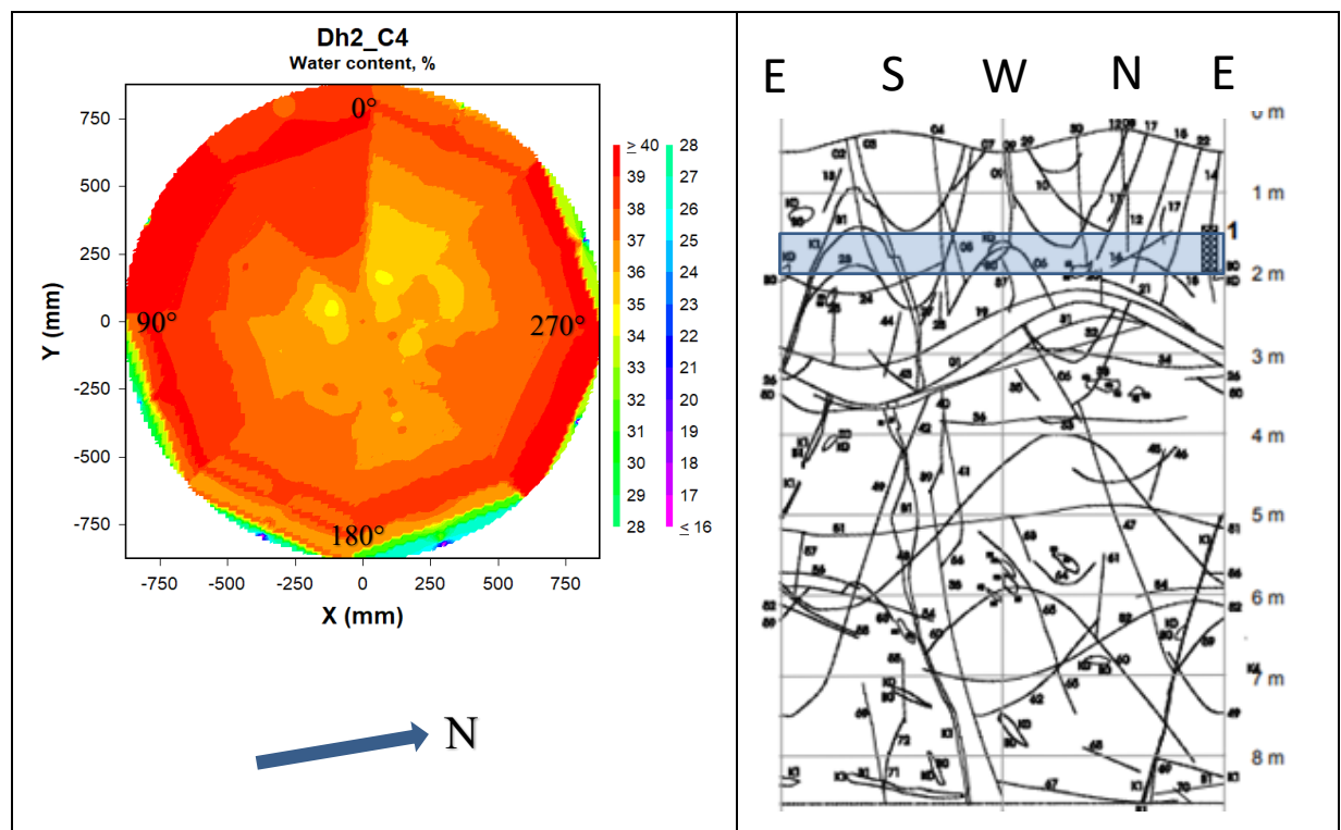
Figure 6-2. Left: Contour plot showing the water content distribution in block C4 in deposition hole 2. Right: Fracture mapping in deposition hole No 2. Water bearing fractures are marked with shaded areas, (Rhén and Forsmark 2001). The blue rectangle indicates the approximate position of block C4 relative to the fractures.
