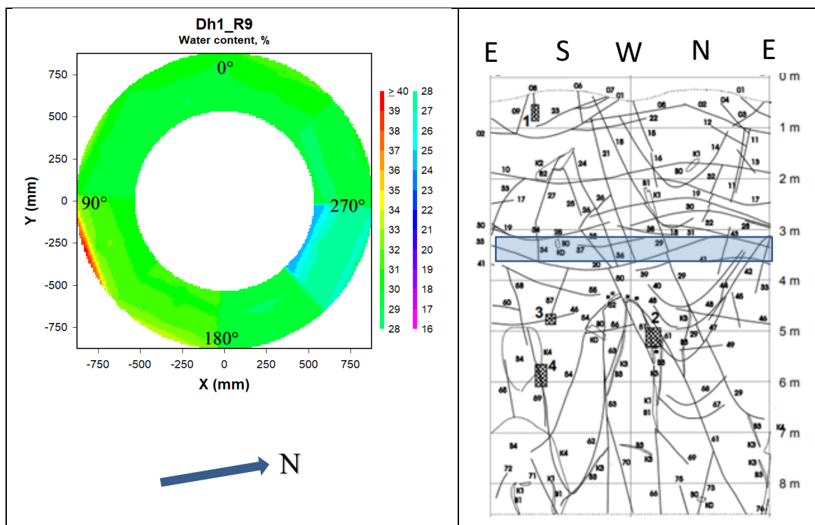
Figure 7-6. Left: Contour plot showing the water content distribution in block R9 in deposition hole 1. Right: Fracture mapping in deposition hole No 1. Water bearing fractures are marked with shaded areas, (Rhén and Forsmark 2001). The blue rectangle indicates the approximate position of block R9 relative to the fractures.
