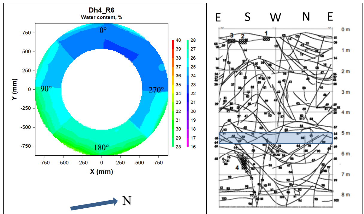
Figure 4-9. Left: Contour plot showing the water content distribution in block R6 in deposition hole 4. The degrees given are those used for sampling. Right: Fracture mapping in deposition hole No 4. Water bearing fractures are marked with shaded areas, (Rhén and Forsmark 2001). The blue rectangle indicates the approximate position of block R6 relative to the fractures.
