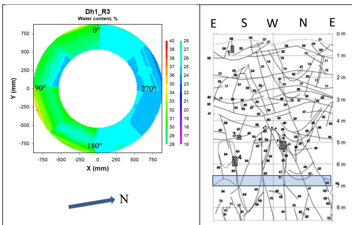
Figure 7-12. Left: Contour plot showing the water content distribution in block R3 in deposition hole 1. Right: Fracture mapping in deposition hole No 1. Water bearing fractures are marked with shaded areas, (Rhén and Forsmark 2001). The blue rectangle indicates the approximate position of block R3 relative to the fractures.
