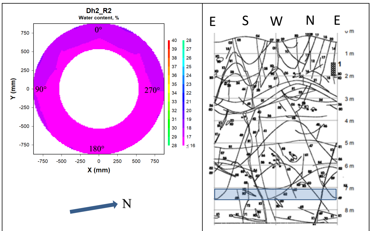
Figure 6-13. Left: Contour plot showing the water content distribution in block R2 in deposition hole 2. Right: Fracture mapping in deposition hole No 2. Water bearing fractures are marked with shaded areas (no such areas in this deposition hole), (Rhén and Forsmark 2001). The blue rectangle indicates the approximate position of block R2 relative to the fractures.
