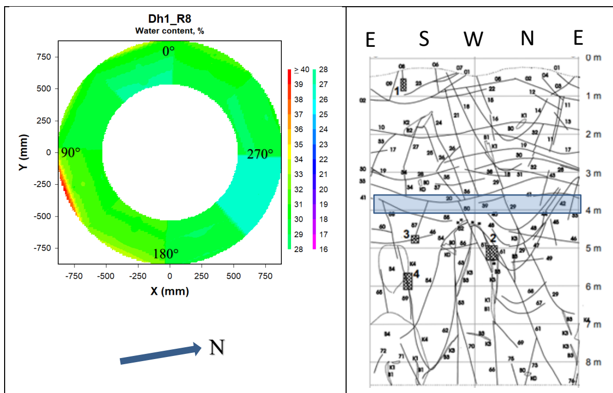
Figure 7-7. Left: Contour plot showing the water content distribution in block R8 in deposition hole 1. Right: Fracture mapping in deposition hole No 1. Water bearing fractures are marked with shaded areas, (Rhén and Forsmark 2001). The blue rectangle indicates the approximate position of block R8 relative to the fractures.
