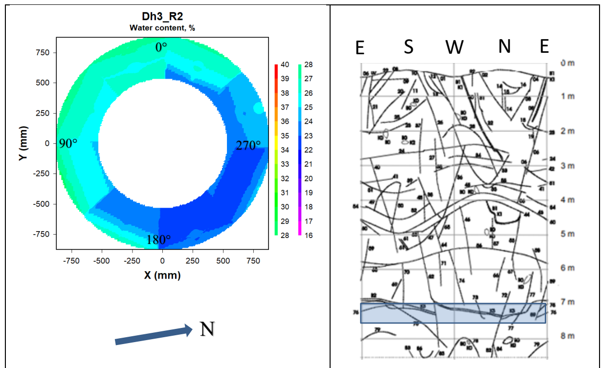
Figure 5-13. Left: Contour plot showing the water content distribution in block R2 in deposition hole 3. Right: Fracture mapping in deposition hole No 3. Water bearing fractures are marked with shaded areas (no such areas in this deposition hole), (Rhén and Forsmark 2001). The blue rectangle indicates the approximate position of block R2 relative to the fractures.
