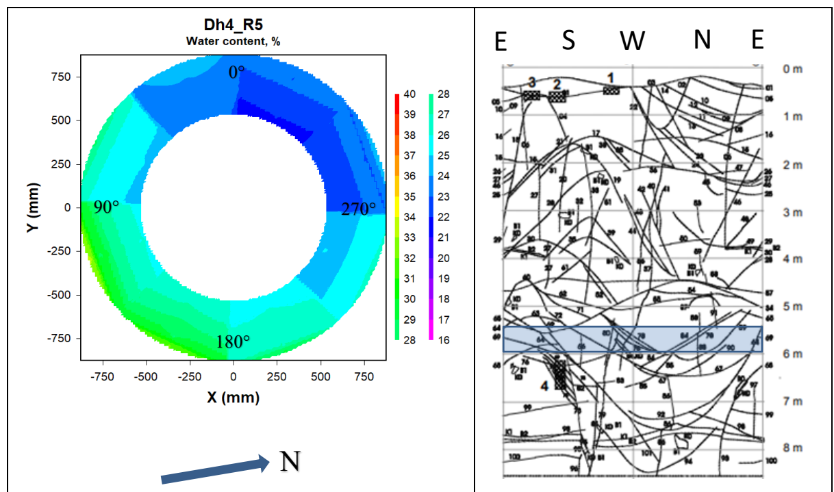
Figure 4-10. Left: Contour plot showing the water content distribution in block R5 in deposition hole 4. The degrees given are those used for sampling. Right: Fracture mapping in deposition hole No 4. Water bearing fractures are marked with shaded areas, (Rhén and Forsmark 2001). The blue rectangle indicates the approximate position of block R5 relative to the fractures.
