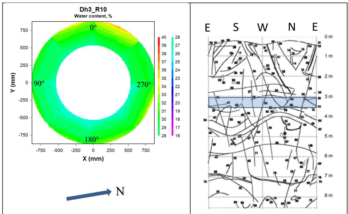
Figure 5-5. Left: Contour plot showing the water content distribution in block R10 in deposition hole 3. Right: Fracture mapping in deposition hole No 3. Water bearing fractures are marked with shaded areas (no such areas in this deposition hole), (Rhén and Forsmark 2001). The blue rectangle indicates the approximate position of block R10 relative to the fractures.
