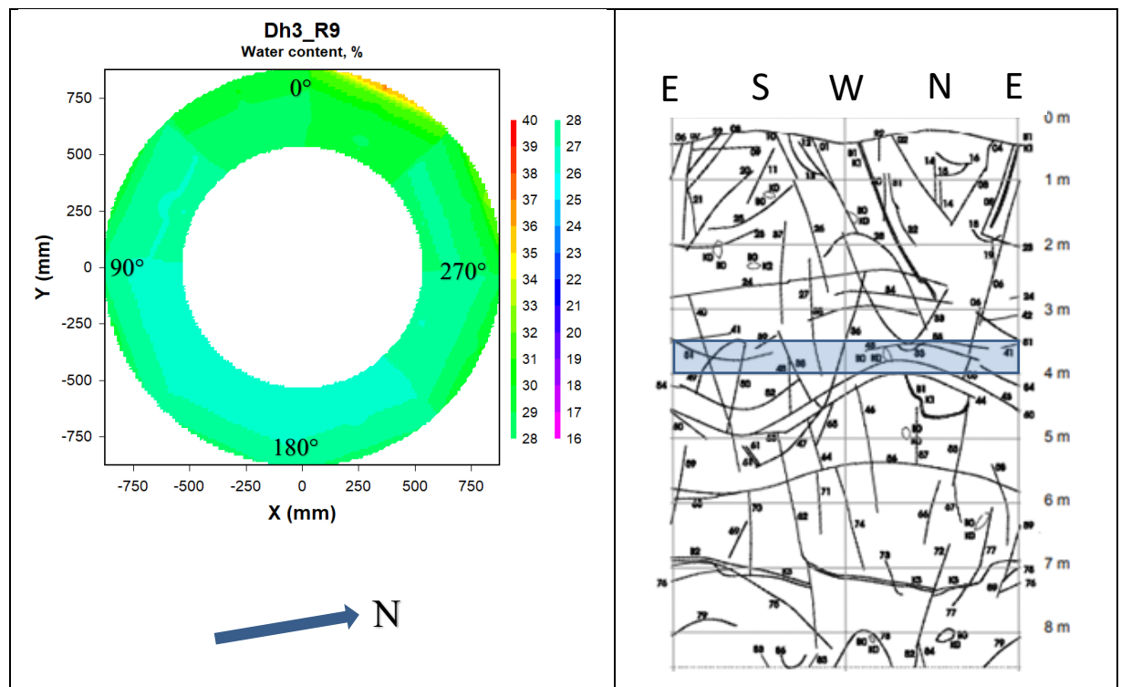
Figure 5-6. Left: Contour plot showing the water content distribution in block R9 in deposition hole 3. Right: Fracture mapping in deposition hole No 3. Water bearing fractures are marked with shaded areas (no such areas in this deposition hole), (Rhén and Forsmark 2001). The blue rectangle indicates the approximate position of block R9 relative to the fractures.
