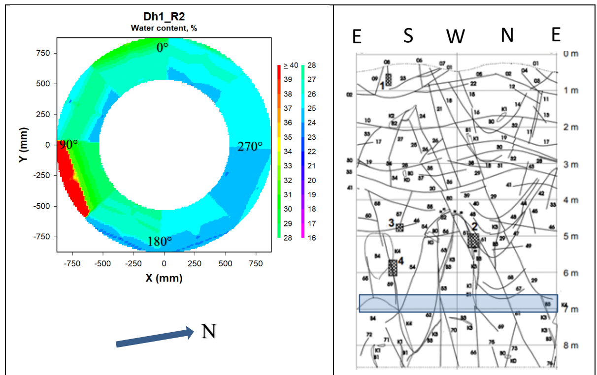
Figure 7-13. Left: Contour plot showing the water content distribution in block R2 in deposition hole 1. Right: Fracture mapping in deposition hole No 1. Water bearing fractures are marked with shaded areas, (Rhén and Forsmark 2001). The blue rectangle indicates the approximate position of block R2 relative to the fractures.
