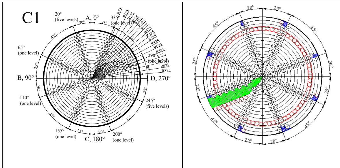
Figure 3-2. Sampling of cylindrical-shaped block. Left: Cores were taken in eight directions at different radius. Right: Extra cores (red) were drilled to loosen the buffer from the deposition hole. A large sample (green) was taken for further investigations in the laboratory and extra samples (blue) were taken close to the rock wall to determine the water content and density distribution here.
