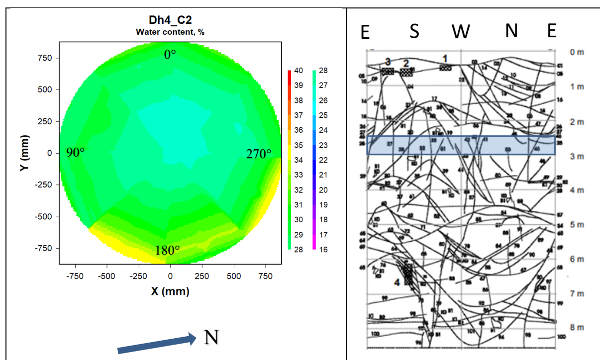
Figure 4-4. Left: Contour plot showing the water content distribution in block C2 in deposition hole 4. The degrees given are those used for sampling. Right: Fracture mapping in deposition hole No 4. Water bearing fractures are marked with shaded areas, (Rhén and Forsmark 2001). The blue rectangle indicates the approximate position of block C2 relative to the fractures.
