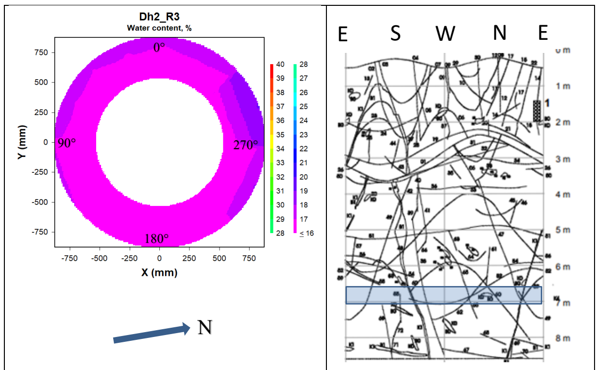
Figure 6-12. Left: Contour plot showing the water content distribution in block R3 in deposition hole 2. Right: Fracture mapping in deposition hole No 2. Water bearing fractures are marked with shaded areas (no such areas in this deposition hole), (Rhén and Forsmark 2001). The blue rectangle indicates the approximate position of block R3 relative to the fractures.
