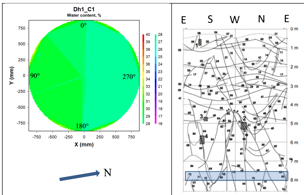
Figure 7-15. Left: Contour plot showing the water content distribution in block C1 in deposition hole 1. Right: Fracture mapping in deposition hole No 1. Water bearing fractures are marked with shaded areas, (Rhén and Forsmark 2001). The blue rectangle indicates the approximate position of block C1 relative to the fractures.
