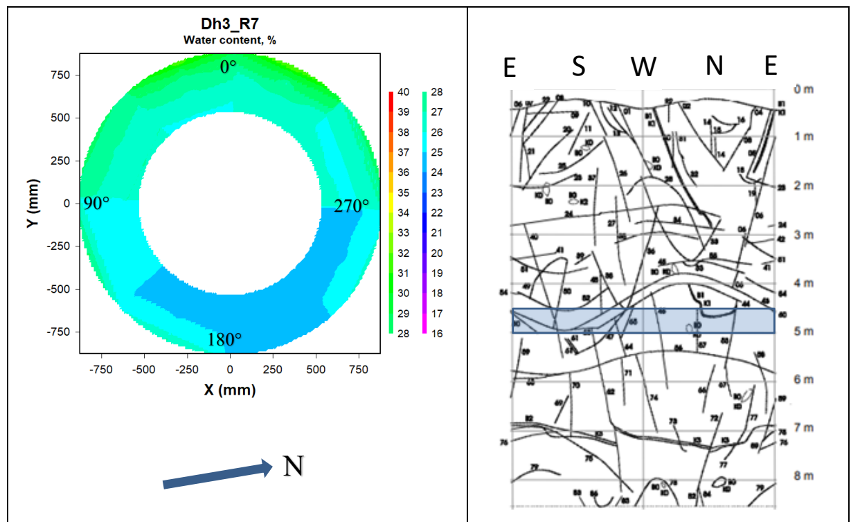
Figure 5-8. Left: Contour plot showing the water content distribution in block R7 in deposition hole 3. Right: Fracture mapping in deposition hole No 3. Water bearing fractures are marked with shaded areas (no such areas in this deposition hole), (Rhén and Forsmark 2001). The blue rectangle indicates the approximate position of block R7 relative to the fractures.
