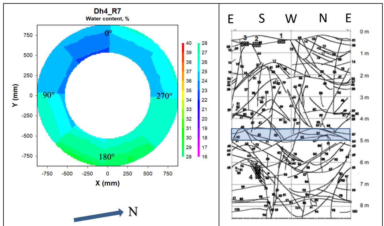
Figure 4-8. Left: Contour plot showing the water content distribution in block R7 in deposition hole 4. The degrees given are those used for sampling. Right: Fracture mapping in deposition hole No 4. Water bearing fractures are marked with shaded areas, (Rhén and Forsmark 2001). The blue rectangle indicates the approximate position of block R7 relative to the fractures.
