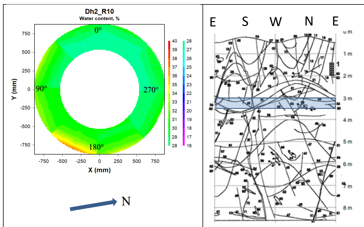
Figure 6-5. Left: Contour plot showing the water content distribution in block R10 in deposition hole 2. Right: Fracture mapping in deposition hole No 2. Water bearing fractures are marked with shaded areas (no such areas in this deposition hole), (Rhén and Forsmark 2001). The blue rectangle indicates the approximate position of block R10 relative to the fractures.
