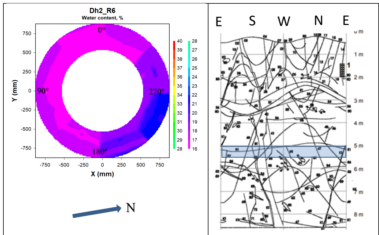
Figure 6-9. Left: Contour plot showing the water content distribution in block R6 in deposition hole 2. Right: Fracture mapping in deposition hole No 2. Water bearing fractures are marked with shaded areas (no such areas in this deposition hole), (Rhén and Forsmark 2001). The blue rectangle indicates the approximate position of block R6 relative to the fractures.
