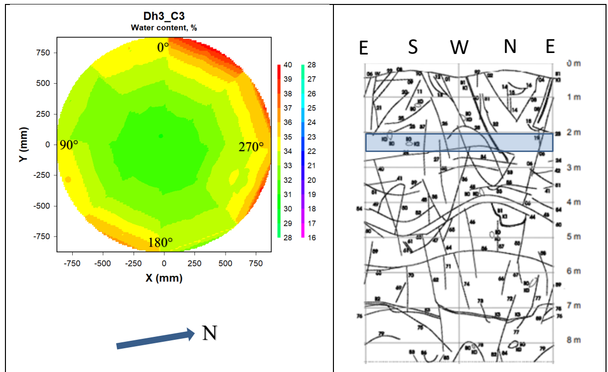
Figure 5-3. Left: Contour plot showing the water content distribution in block C3 in deposition hole 3. Right: Fracture mapping in deposition hole No 3. Water bearing fractures are marked with shaded areas (no such areas in this deposition hole), (Rhén and Forsmark 2001). The blue rectangle indicates the approximate position of block C3 relative to the fractures.
