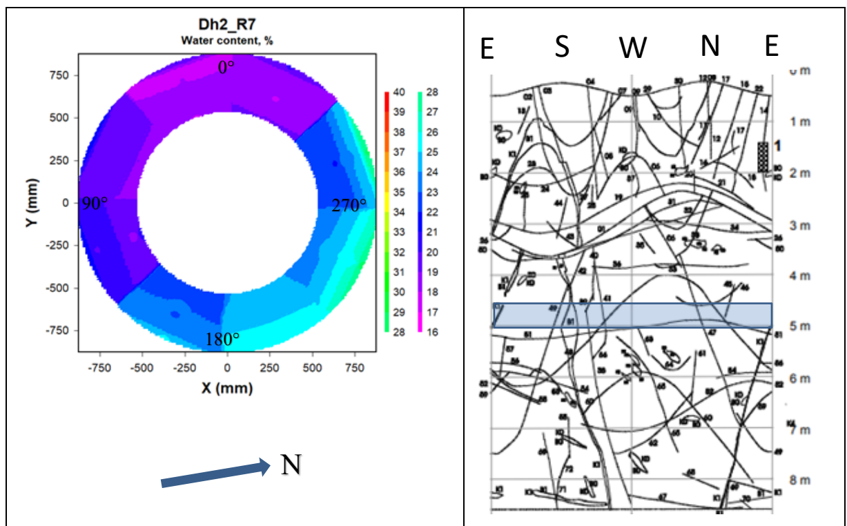
Figure 6-8. Left: Contour plot showing the water content distribution in block R7 in deposition hole 2. Right: Fracture mapping in deposition hole No 2. Water bearing fractures are marked with shaded areas (no such areas in this deposition hole), (Rhén and Forsmark 2001). The blue rectangle indicates the approximate position of block R7 relative to the fractures.
