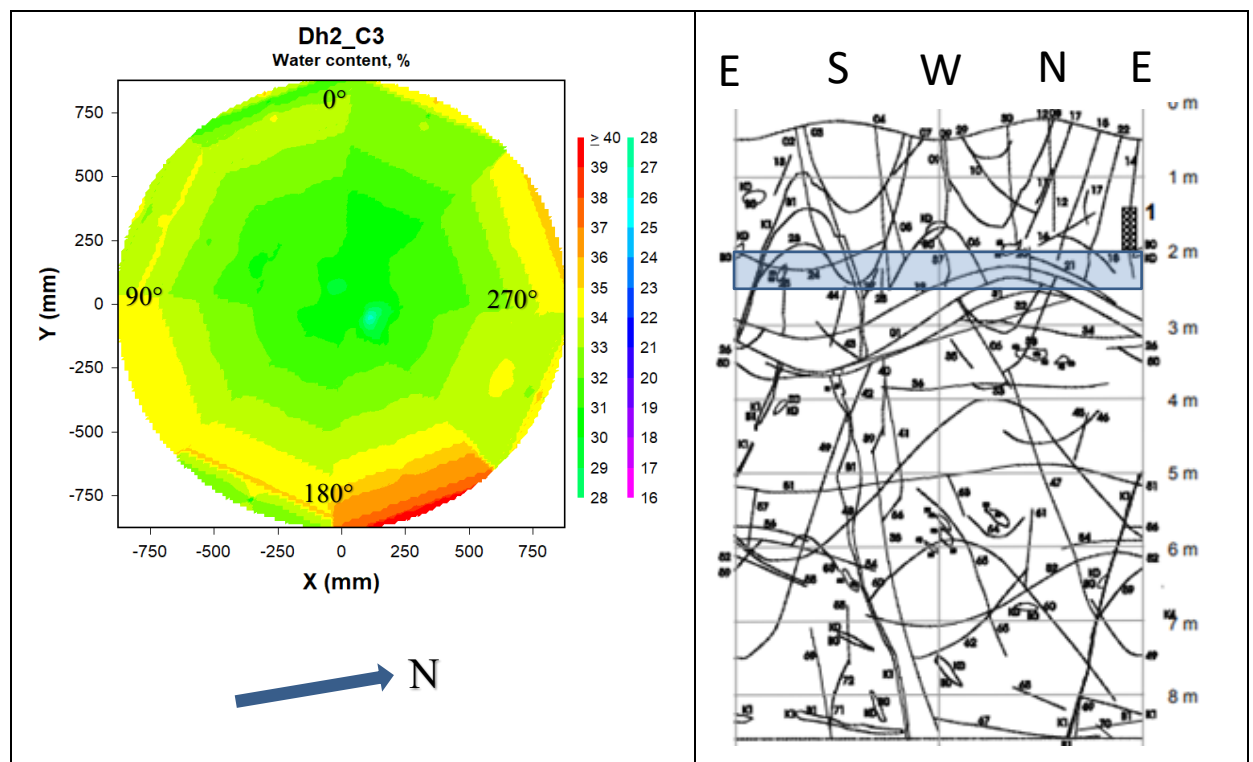
Figure 6-3. Left: Contour plot showing the water content distribution in block C3 in deposition hole 2. Right: Fracture mapping in deposition hole No 2. Water bearing fractures are marked with shaded areas, (Rhén and Forsmark 2001). The blue rectangle indicates the approximate position of block C3 relative to the fractures.
