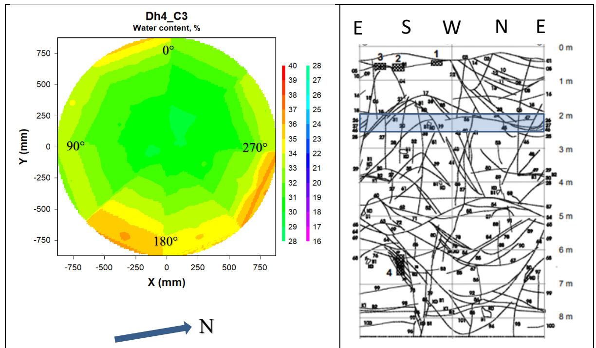
Figure 4-3. Left: Contour plot showing the water content distribution in block C3 in deposition hole 4. The degrees given are those used for sampling. Right: Fracture mapping in deposition hole No 4. Water bearing fractures are marked with shaded areas, (Rhén and Forsmark 2001). The blue rectangle indicates the approximate position of block C3 relative to the fractures.
