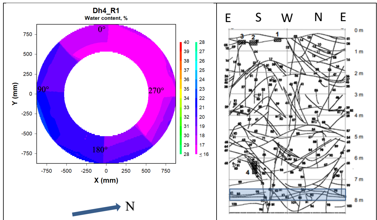
Figure 4-14. Left: Contour plot showing the water content distribution in block R1 in deposition hole 4. The degrees given are those used for sampling. Right: Fracture mapping in deposition hole No 4. Water bearing fractures are marked with shaded areas, (Rhén and Forsmark 2001). The blue rectangle indicates the approximate position of block R1 relative to the fractures.
