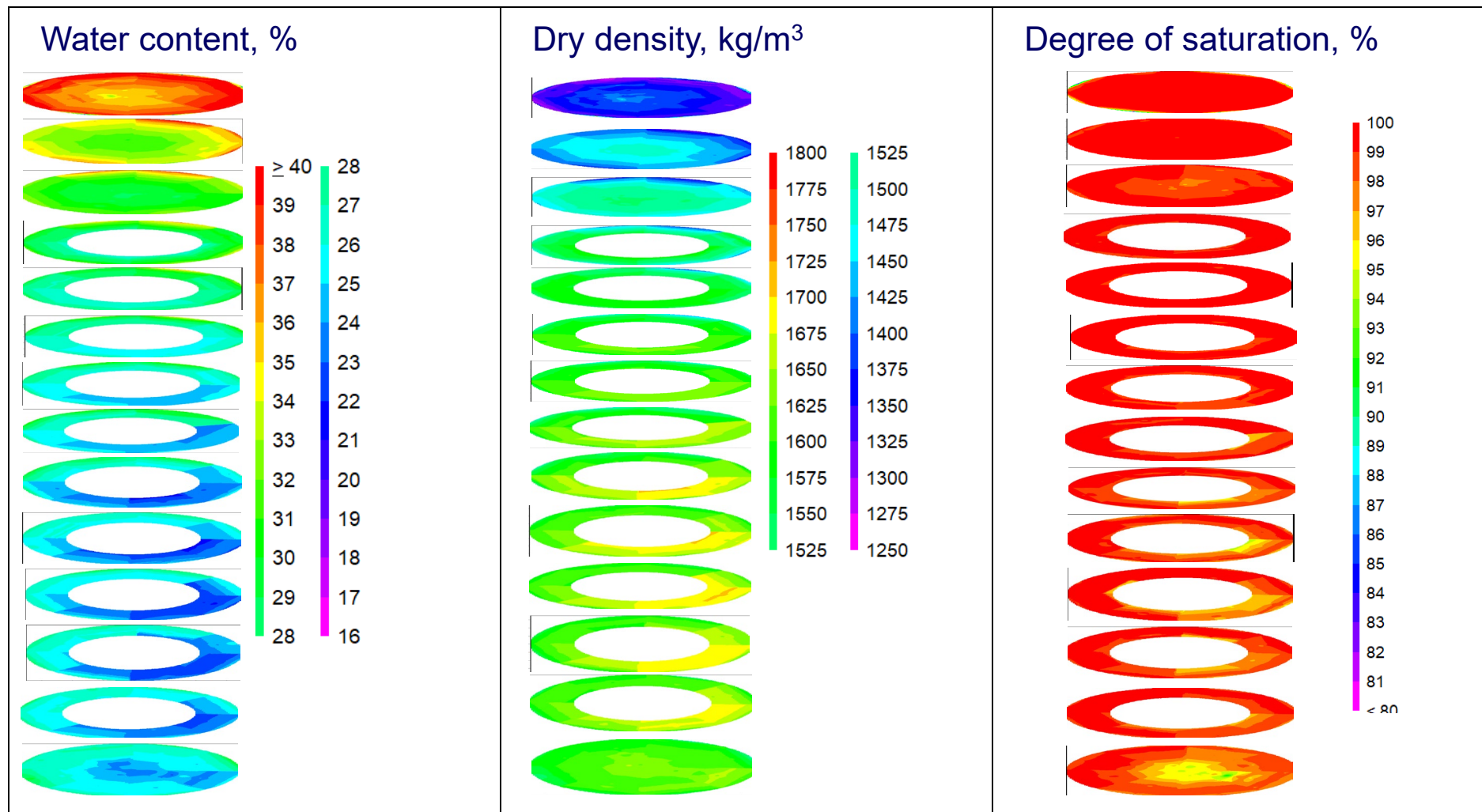
Figure 5-16. Compressed contour plots of every single block in Dh 3 stacked on each other. Left: the water content distribution (%) Middle: the dry density distribution (kg/m 3 ) Right: the degree of saturation distribution (%).
