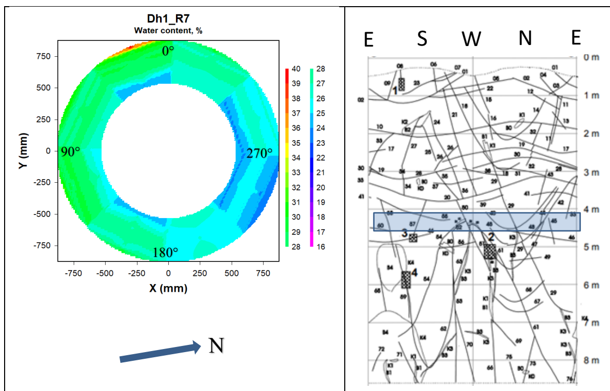
Figure 7-8. Left: Contour plot showing the water content distribution in block R7 in deposition hole 1. Right: Fracture mapping in deposition hole No 1. Water bearing fractures are marked with shaded areas, (Rhén and Forsmark 2001). The blue rectangle indicates the approximate position of block R7 relative to the fractures.
