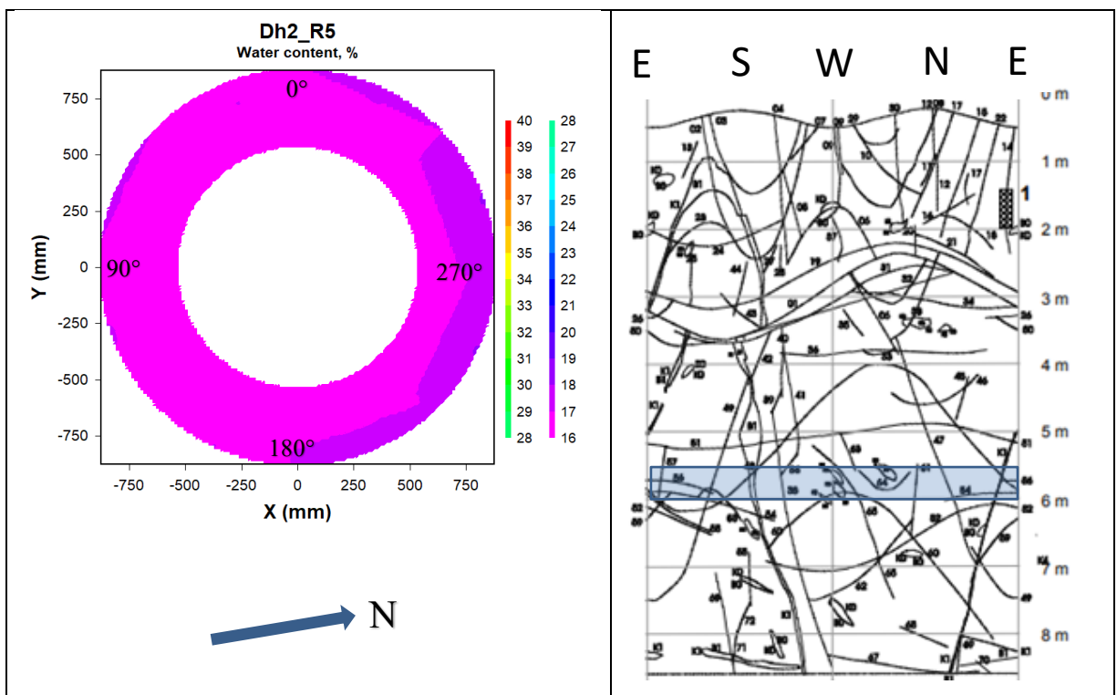
Figure 6-10. Left: Contour plot showing the water content distribution in block R5 in deposition hole 2. Right: Fracture mapping in deposition hole No 2. Water bearing fractures are marked with shaded areas (no such areas in this deposition hole), (Rhén and Forsmark 2001). The blue rectangle indicates the approximate position of block R5 relative to the fractures.
