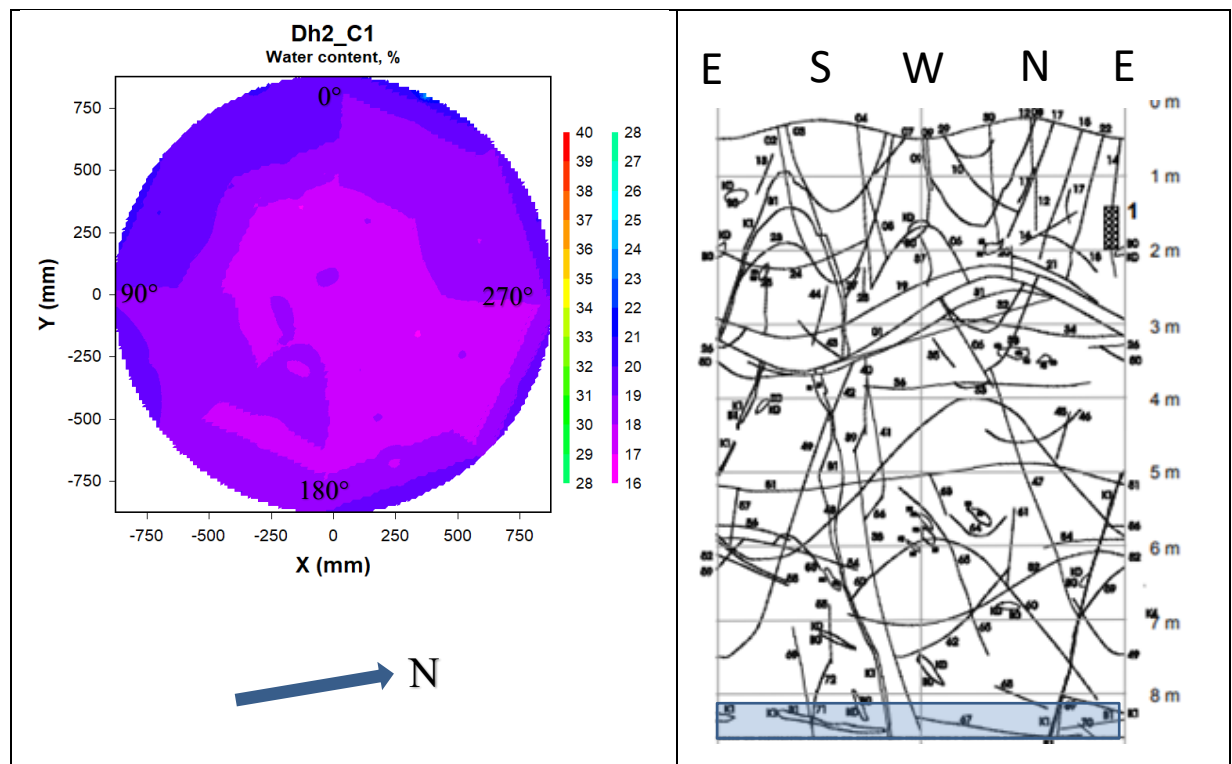
Figure 6-15. Left: Contour plot showing the water content distribution in block C1 in deposition hole 2. Right: Fracture mapping in deposition hole No 2. Water bearing fractures are marked with shaded areas (no such areas in this deposition hole), (Rhén and Forsmark 2001). The blue rectangle indicates the approximate position of block C1 relative to the fractures.
