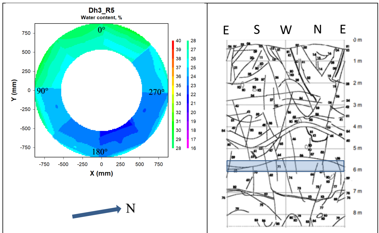
Figure 5-10. Left: Contour plot showing the water content distribution in block R5 in deposition hole 3. Right: Fracture mapping in deposition hole No 3. Water bearing fractures are marked with shaded areas (no such areas in this deposition hole), (Rhén and Forsmark 2001). The blue rectangle indicates the approximate position of block R5 relative to the fractures.
