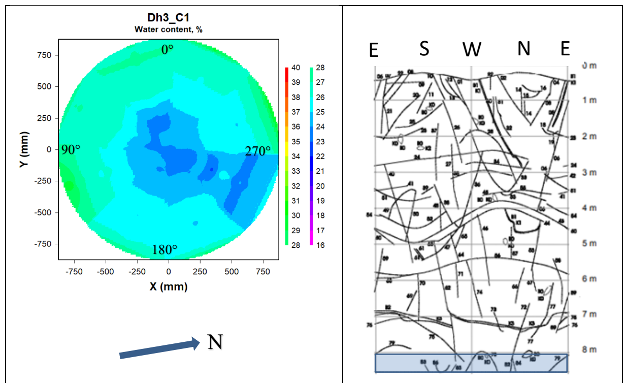
Figure 5-15. Left: Contour plot showing the water content distribution in block C1 in deposition hole 3. Right: Fracture mapping in deposition hole No 3. Water bearing fractures are marked with shaded areas (no such areas in this deposition hole), (Rhén and Forsmark 2001). The blue rectangle indicates the approximate position of block C1 relative to the fractures.
