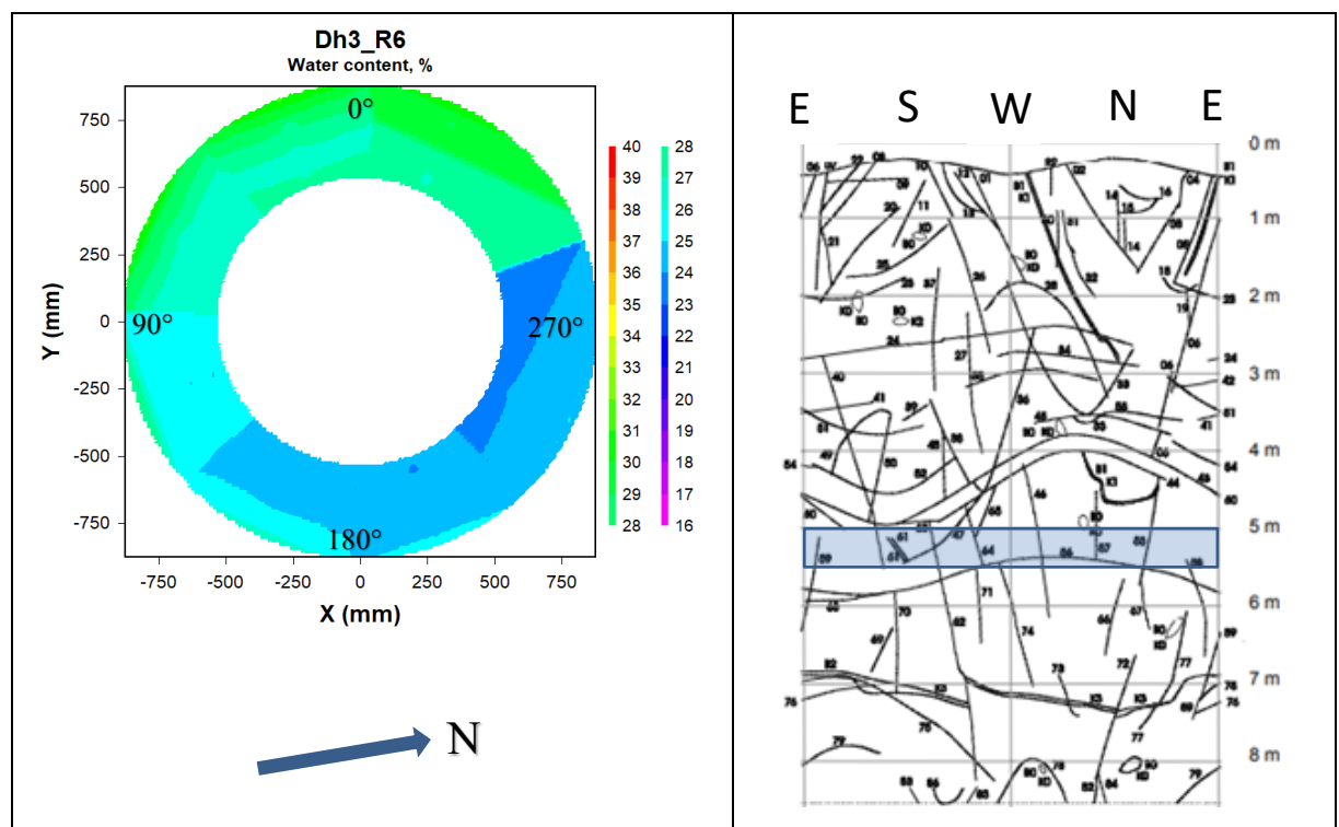
Figure 5-9. Left: Contour plot showing the water content distribution in block R6 in deposition hole 3. Right: Fracture mapping in deposition hole No 3. Water bearing fractures are marked with shaded areas (no such areas in this deposition hole), (Rhén and Forsmark 2001). The blue rectangle indicates the approximate position of block R6 relative to the fractures.
