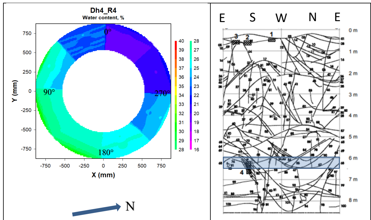
Figure 4-11. Left: Contour plot showing the water content distribution in block R4 in deposition hole 4. The degrees given are those used for sampling. Right: Fracture mapping in deposition hole No 4. Water bearing fractures are marked with shaded areas, (Rhén and Forsmark 2001). The blue rectangle indicates the approximate position of block R4 relative to the fractures.
