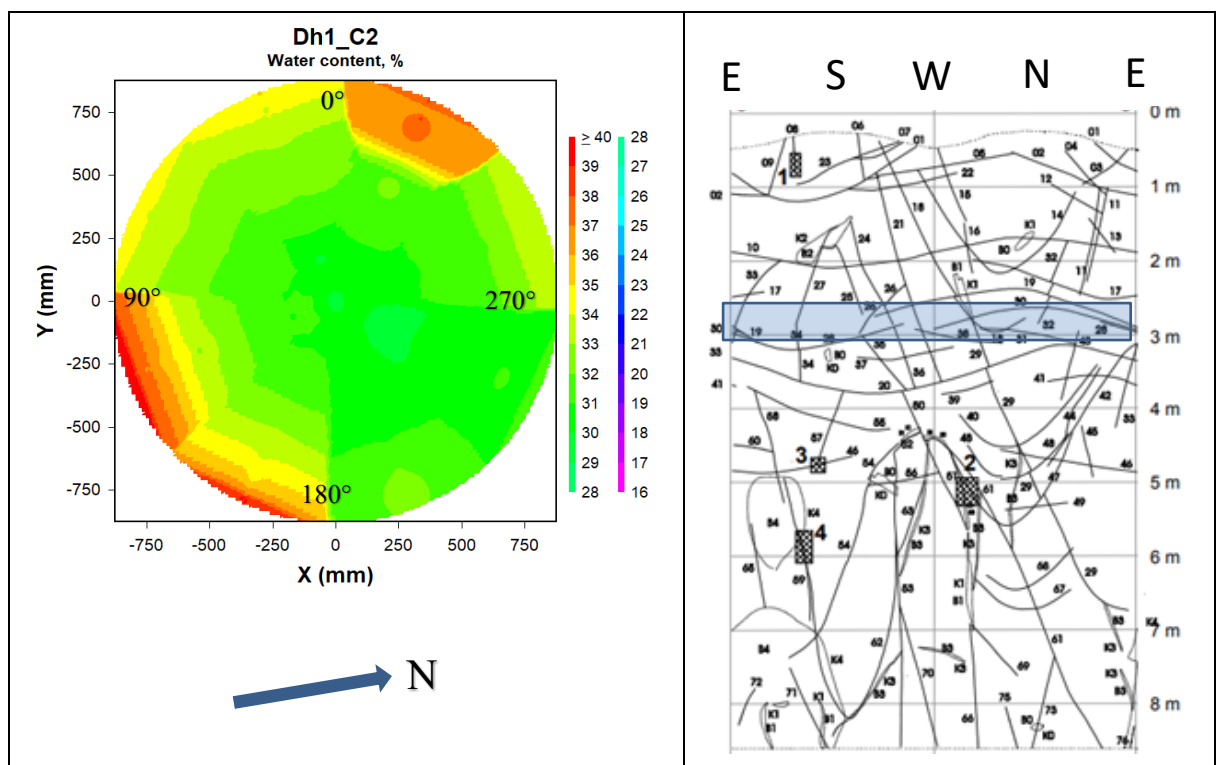
Figure 7-4. Left: Contour plot showing the water content distribution in block C2 in deposition hole 1. Right: Fracture mapping in deposition hole No 1. Water bearing fractures are marked with shaded areas, (Rhén and Forsmark 2001). The blue rectangle indicates the approximate position of block C2 relative to the fractures.
