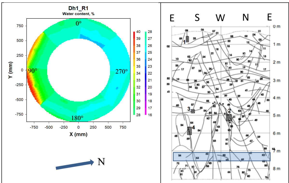
Figure 7-14. Left: Contour plot showing the water content distribution in block R1 in deposition hole 1. Right: Fracture mapping in deposition hole No 1. Water bearing fractures are marked with shaded areas, (Rhén and Forsmark 2001). The blue rectangle indicates the approximate position of block R1 relative to the fractures.
