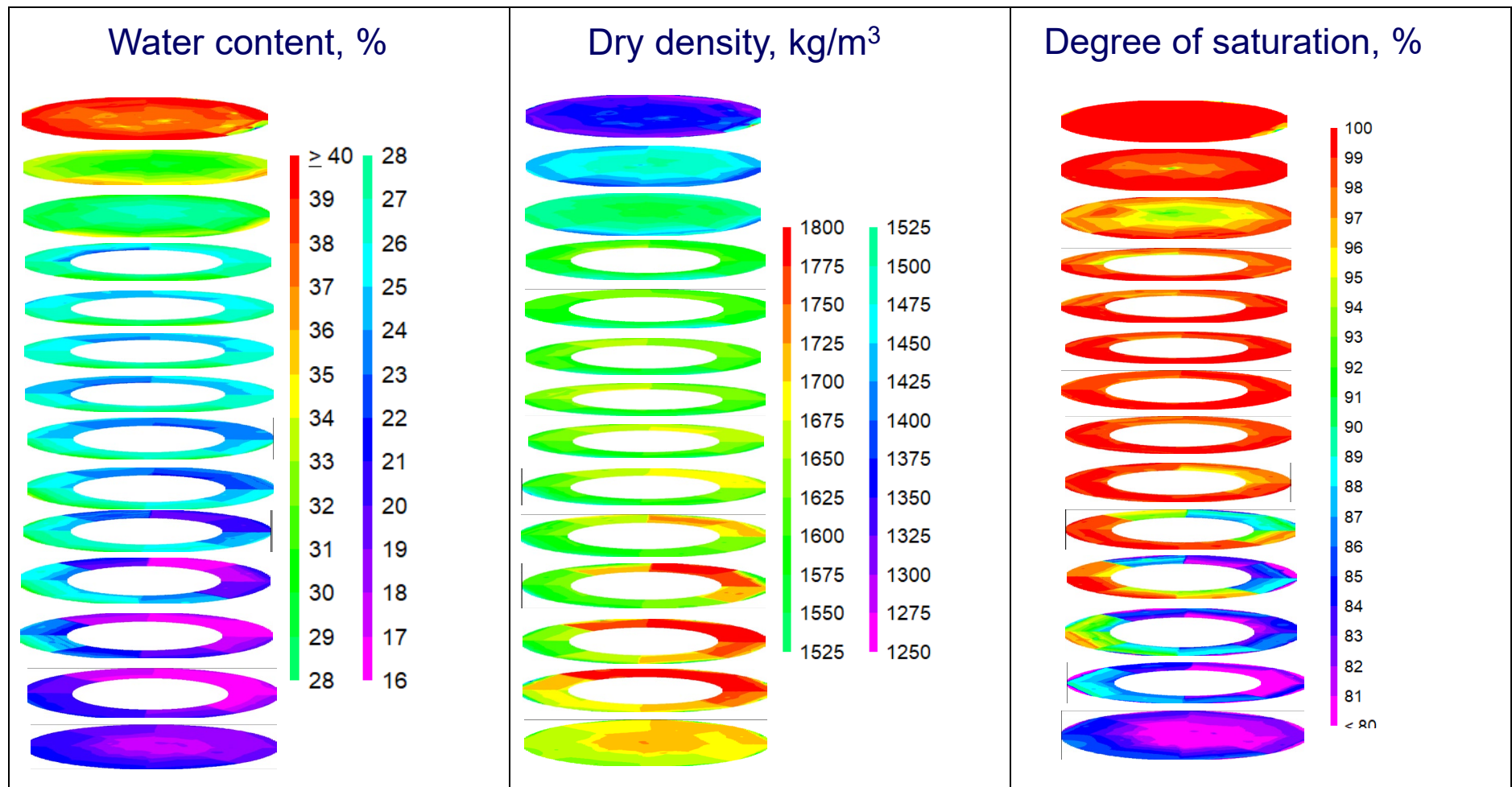
Figure 4-16. Compressed contour plots of every single block in Dh 4 stacked on each other. Left: the water content distribution (%) Middle: the dry density distribution (kg/m³) Right: the degree of saturation distribution (%).
