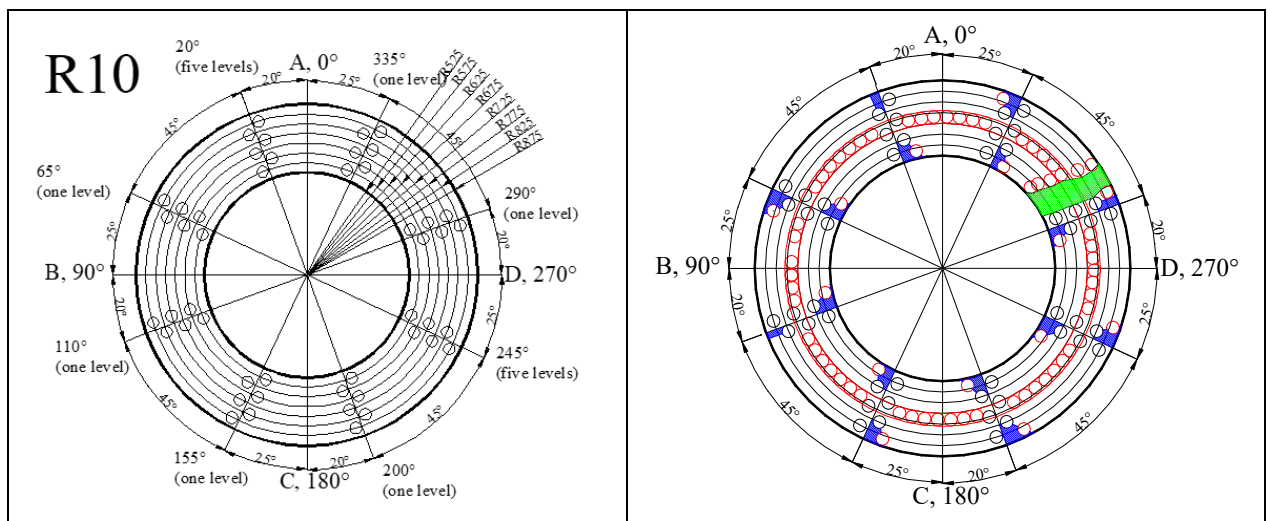
Figure 3-3. Sampling of ring-shaped block. Left: Cores were taken in eight directions at different radius. Right: Extra cores (red) were drilled to loosen the buffer from the deposition hole. A large sample (green) was taken for further investigations in the laboratory and extra samples (blue) were taken close to the canister and close to the rock wall to determine the water content and density distribution here.
