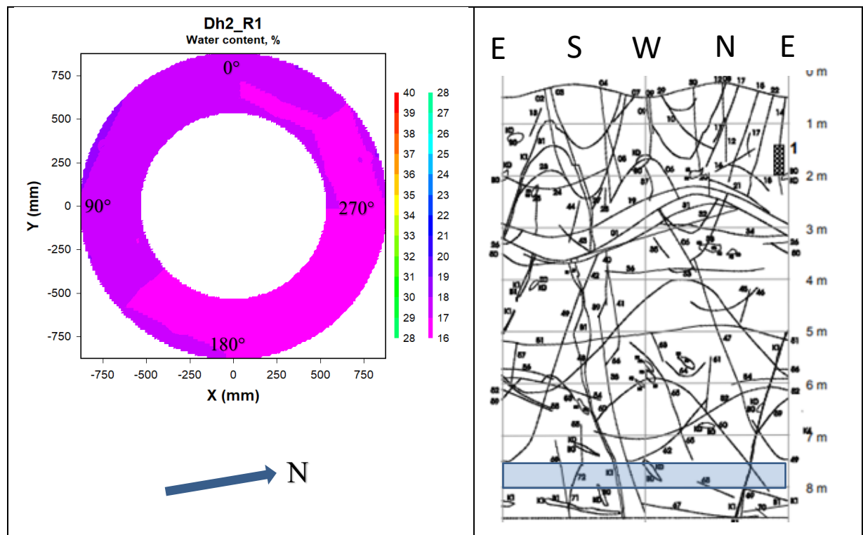
Figure 6-14. Left: Contour plot showing the water content distribution in block R1 in deposition hole 2. Right: Fracture mapping in deposition hole No 2. Water bearing fractures are marked with shaded areas (no such areas in this deposition hole), (Rhén and Forsmark 2001). The blue rectangle indicates the approximate position of block R1 relative to the fractures.
