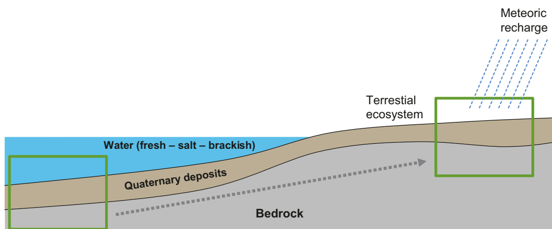
Figure 6-4. A hypothetical cross-section of the Forsmark area today, illustrating the spatial gradient that can be extrapolated and translated into a succession of landscape maturation for the future. The left box may represent the conditions soon after the deglaciation (8800 BC), whereas the right box represents conditions in the most elevated parts of the area, which have been exposed to meteoric recharge and chemical weathering for several thousands of years. Figure from /Tröjbom and Grolander 2010/.
