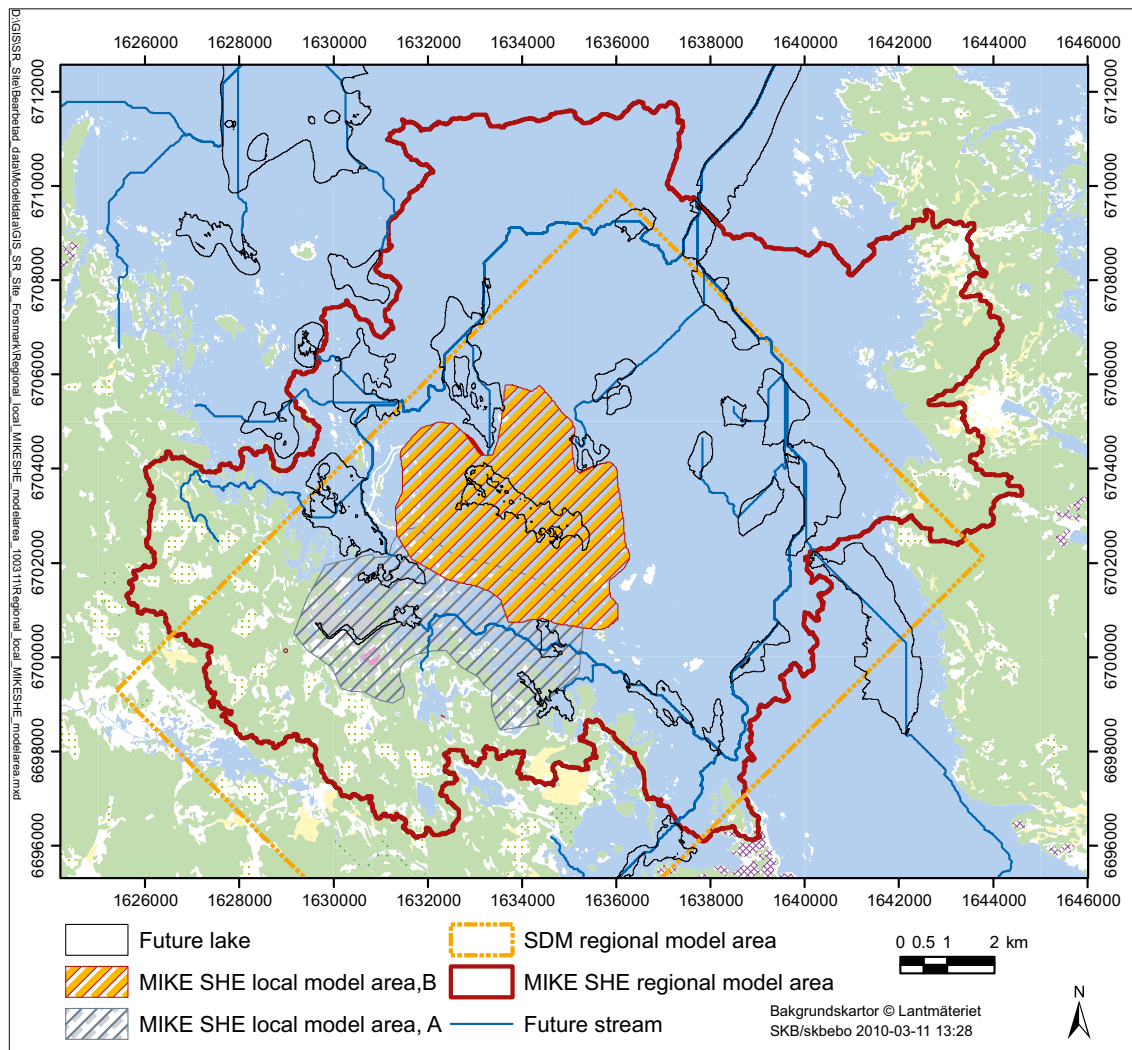
Figure 7-3. The regional and local MIKE SHE model areas. In the figure, the site descriptive modelling (SDM) regional model area and the future lakes and streams are also marked. Figure from /Bosson et al. 2010/.
