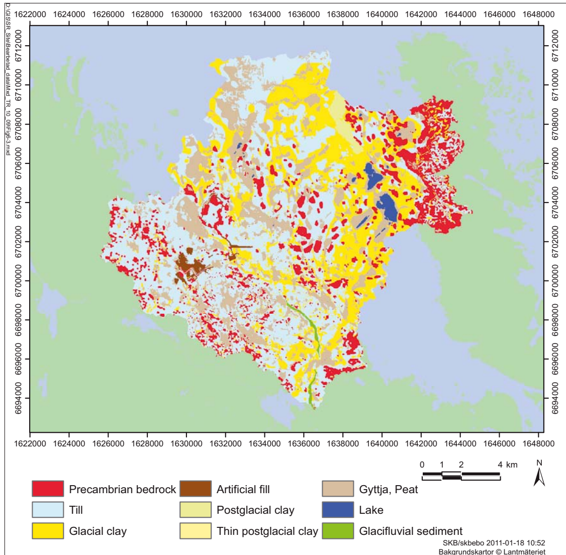
Figure 6-3. Surface distribution of regolith at 10,000 AD according to the Coupled regolith-lake development model /Brydsten and Strömngren 2010/. Most of the postglacial clay is eroded and transported out of the area. The only larger remaining area of postglacial clay is in the former marine basin Gräsörännan , in the north-central part of the figure. Figure from /Brydsten and Strömngren 2010/.
