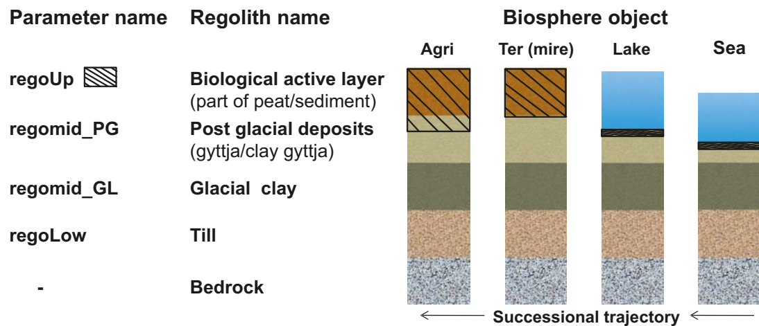
Figure 9-1. Conceptual model of generalized distribution of regolith for different types of biosphere objects at Forsmark. The different depths of the various regolith layers in profiles are also seen in the landscape pictures, which represent a generalized succession trajectory from sea to wetland that is later converted to agricultural land by draining. In the radionuclide model, the postglacial and glacial clay deposits are combined in regard to the radionuclide inventory.
