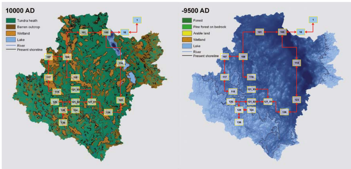
Figure 7-12. Figure illustrating the landscape model under periglacial and submerged conditions. The boxes show biosphere objects (with id numbers) at their approximate locations in the landscape, and red arrows indicate the surface water flow paths connecting the objects. The blue boxes represent Öregrundsgrepen (object 10) and the model area outlet, the Baltic Sea (object 1).
