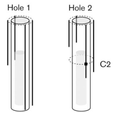
Biaxial stressmeter C2 Maximum stress increase and stress reduction in plane perpendicular to borehole axis
