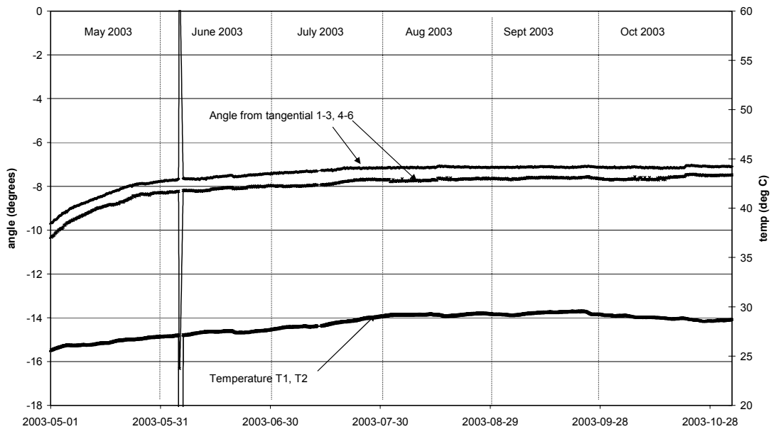
Biaxial stressmeter A2 Orientation of maximum stress increase in plane perpendicular to borehole axis
