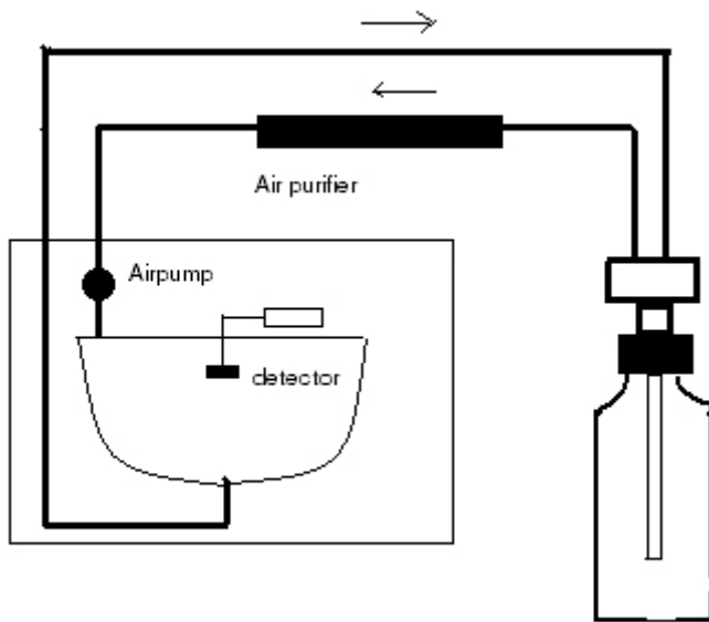
Figure 4-1. Schematic picture of the RAD-7 H 2 O accessory (after /DurrIDGE Company 2000/).
