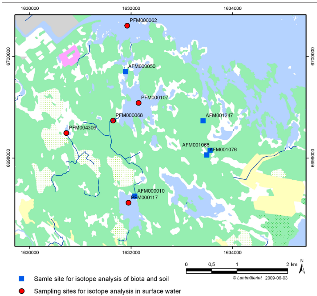
Figure 3-2. The sampling locations for soil, biota and surface water samples collected for determinations of radium, uranium and thorium isotopes.
