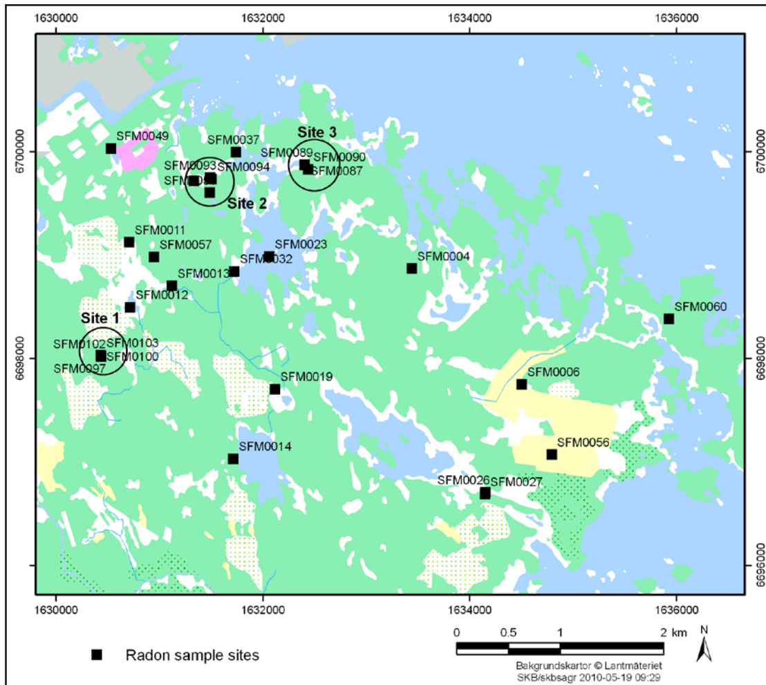
Figure 3-1. The sampling locations for the radon measurements in near surface groundwater. SFM0013, SFM0014, SFM0019 and SFM0026 have been sampled both in June 2009 and October 2008. Site 1, Site 2 and Site 3 represent clusters of monitoring wells, where several wells were samples with different screening depths.
