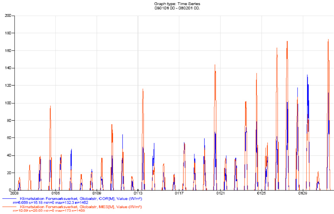
Figure A-13. Global radiation in W/m^2 , 30-min. values, January 2008.
