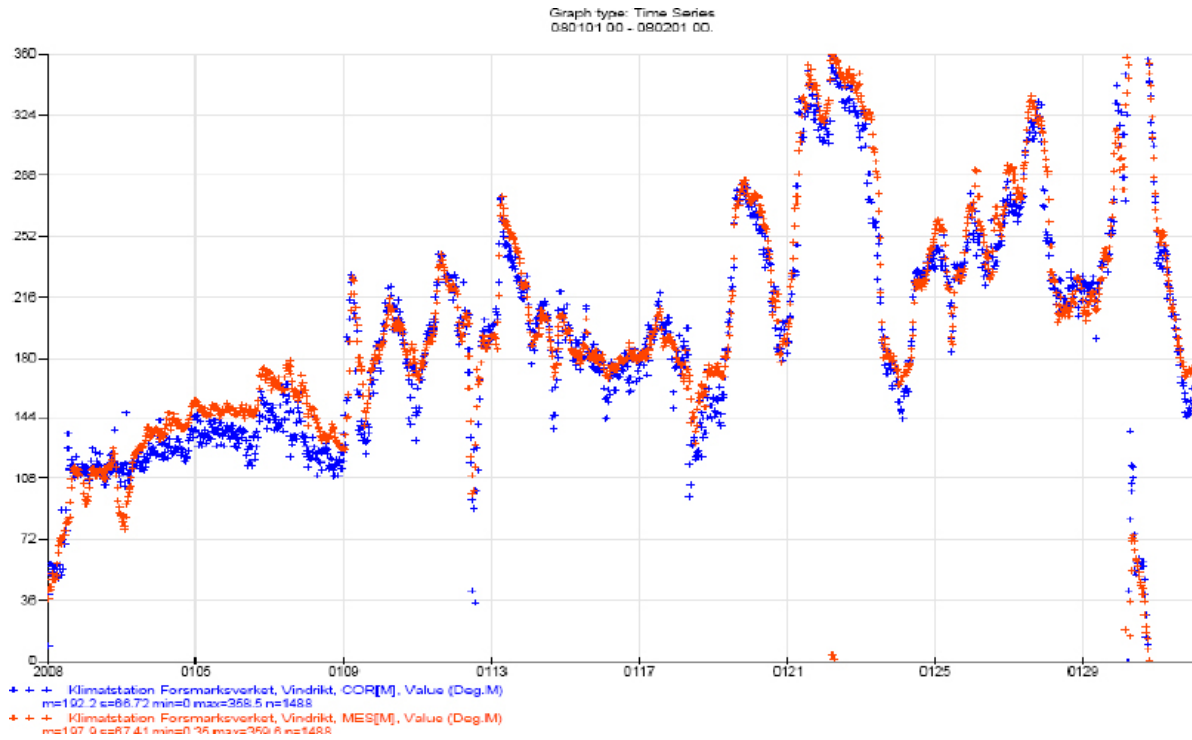
Figure A-11. Wind direction in ^{\circ} , 30-min. values, January 2008.
