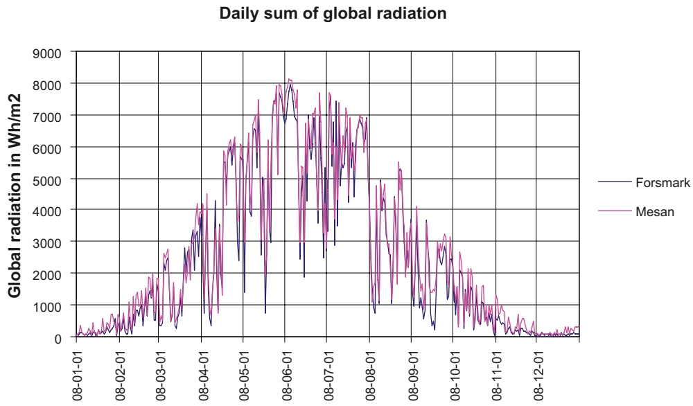
Figure A-5. Global radiation in Wh/m 2 , daily sum, January 2008–December 2008.
