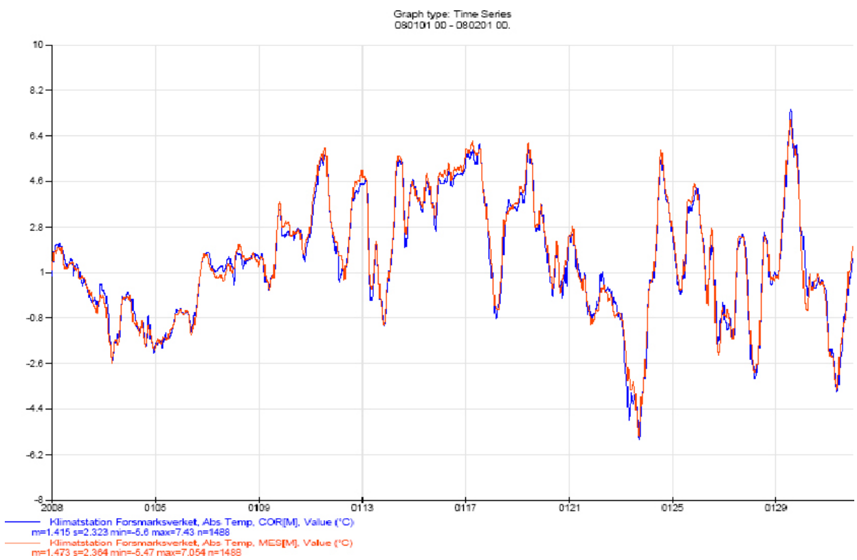
Figure A-8. Temperature in °C, 30-min. value, January 2008.
