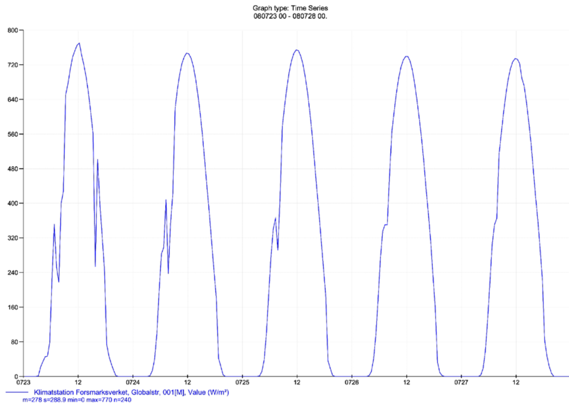
Figure 5-3. Global radiation 23–27 July 2008.
