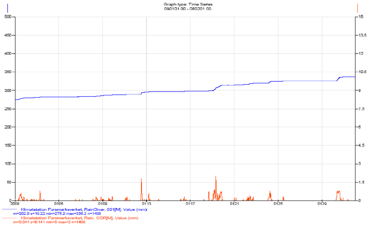
Figure A-7. Precipitation in mm, 30-min. values, January 2008.
