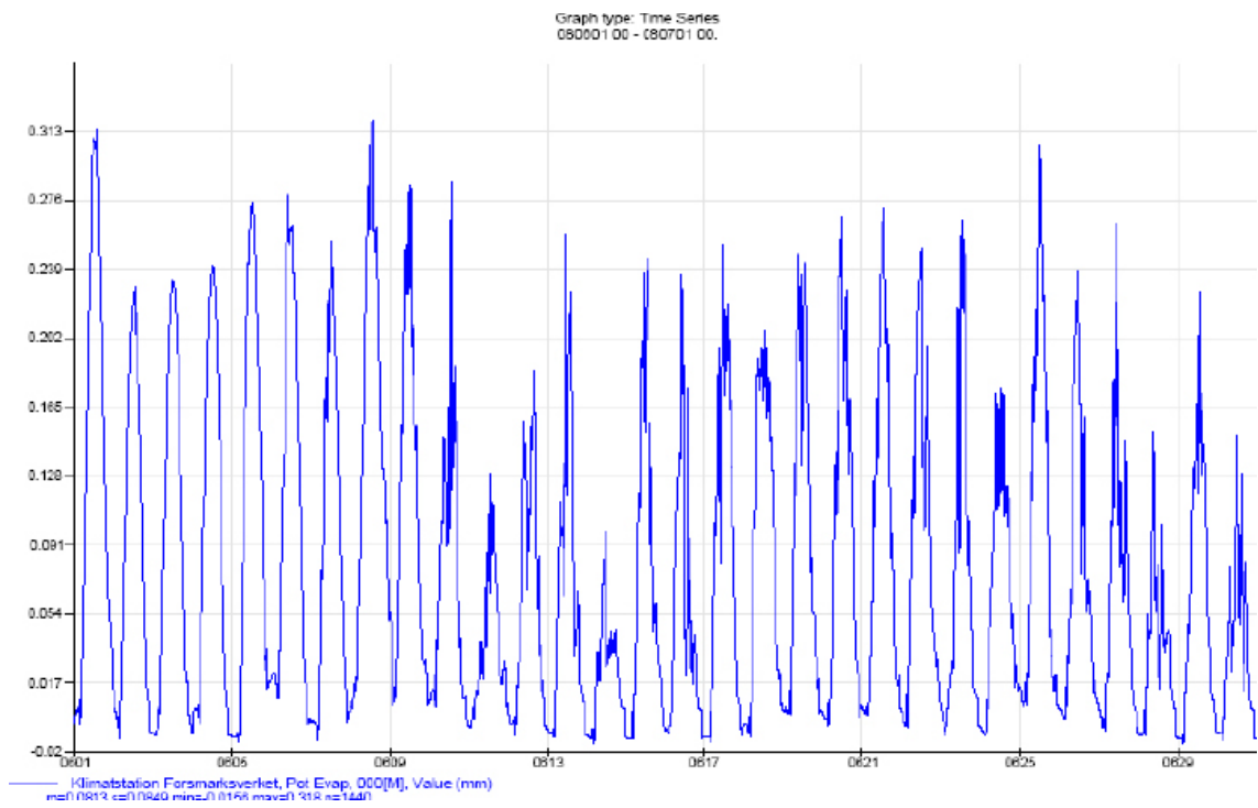
Figure A-14. Potential evapotranspiration in mm, 30-min. values, June 2008.
