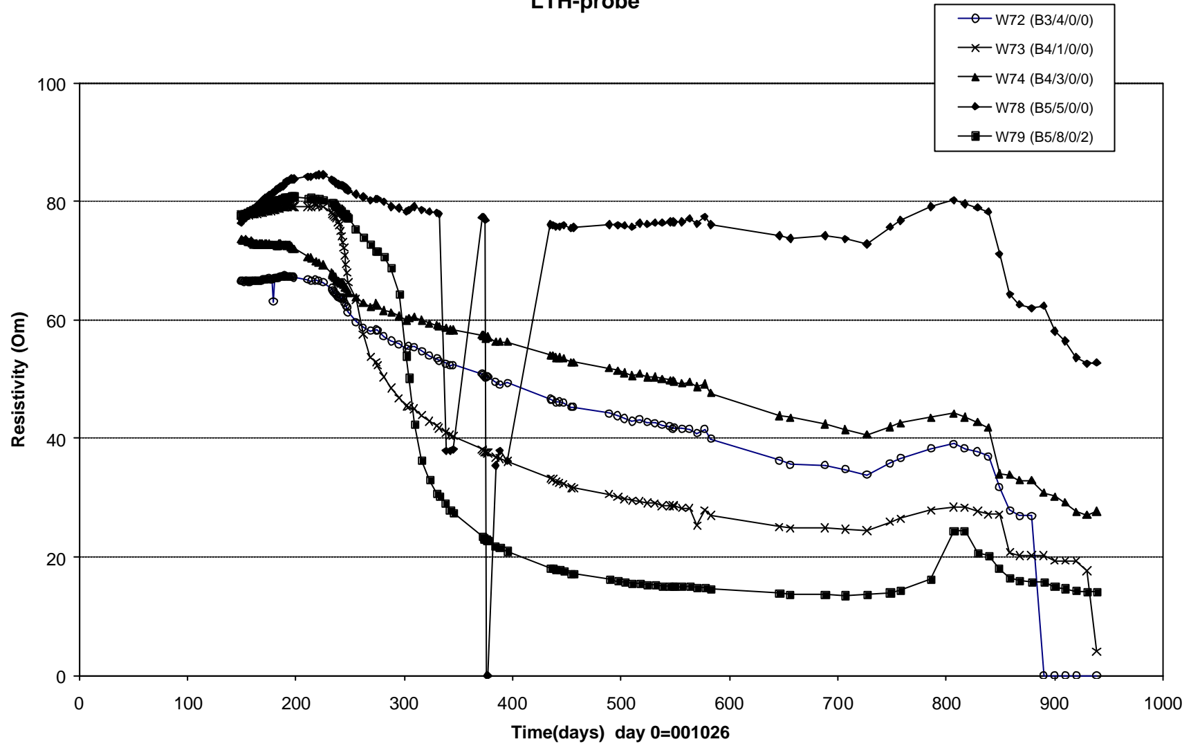
Resistivity in backfill sections B3, B4&B5 (990601-020101) LTH-probe
