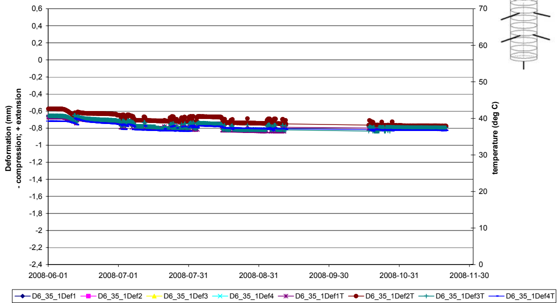
Deformation measurements Borehole D6:3.5(1)
