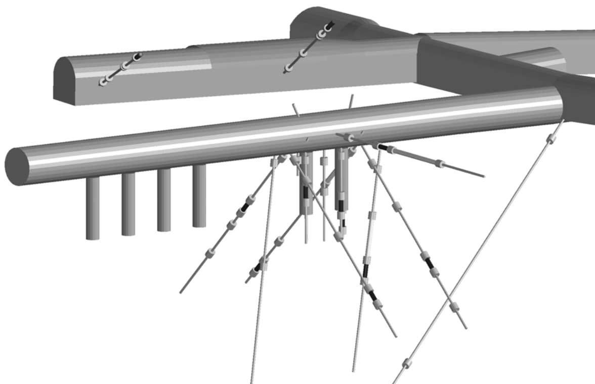
Figure 3. View of the drilled core holes in the Prototype Repository Section II. The length from the I-tunnel to the end of the TBM-tunnel is 90 m. The diameter of the TBM tunnel is 5 m and the diameter of the deposition holes is 1.75 m. The depth of the deposition holes is 8.37 m in the centre and 8.15 m along the deposition hole wall. The diameter of the core holes is 76 mm except for the short core holes in the roof of the TBM tunnel that have a diameter of 56 mm. The monitoring boreholes used in the presentation in this report are located in the inner part of the tunnel surrounding the area with the four innermost canister holes. Also included are two holes drilled from the G-tunnel and the long hole KA3510A drilled from the main tunnel.
