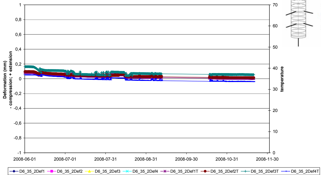
Deformation measurements Borehole D6:3.5(2)
