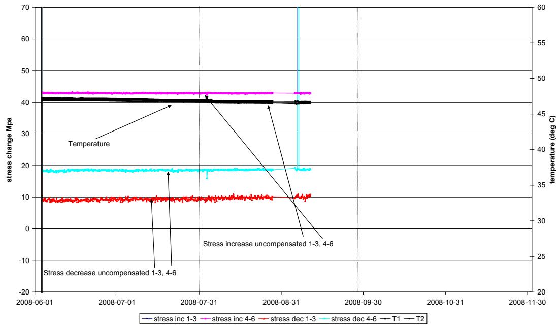
Biaxial stressmeter A5 Maximum stress increase and stress decrease in plane perpendicular to borehole axis
