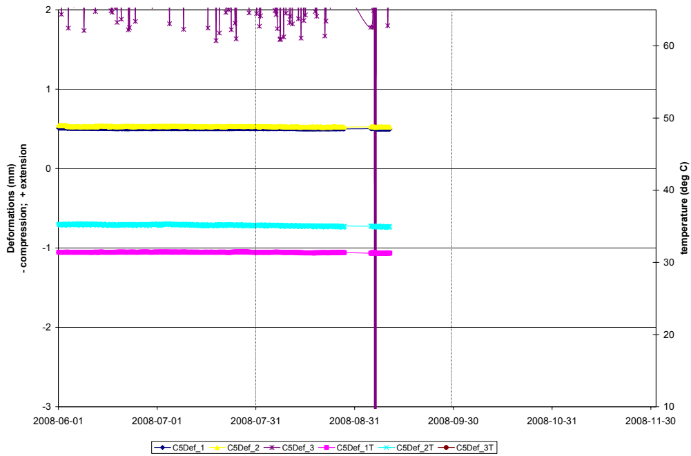
Vertical deformations adjacent to Deposition Hole 5 in borehole C5
