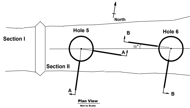
Figure 2.4 Plan view of complementary boreholes.
