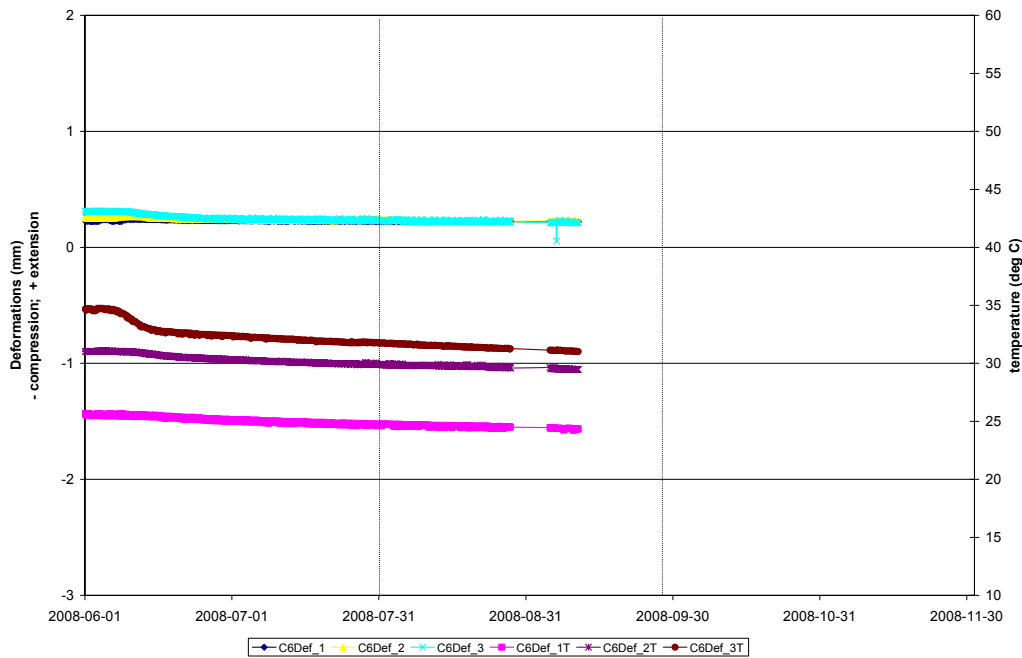
Vertical deformations adjacent to Deposition Hole 6 in borehole C6
