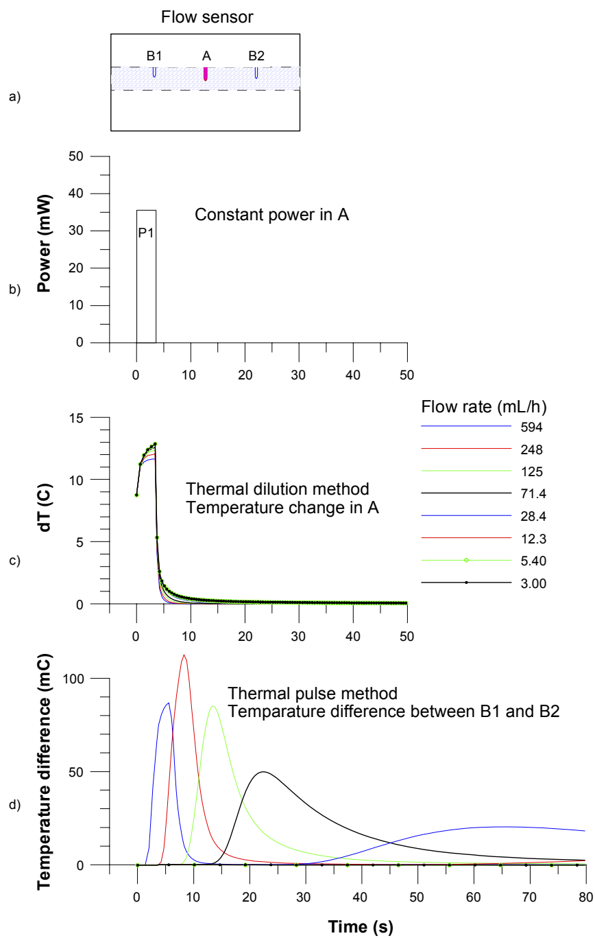
Figure 3-3. Flow measurement, flow rate <600 mL/h.
