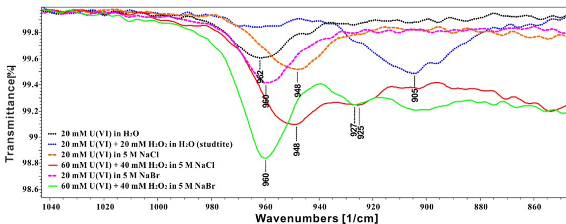
Figure 7. IR spectra of aqueous solutions containing \text{UO}_2^{2+} , \text{H}_2\text{O}_2 , NaBr, or NaCl.
