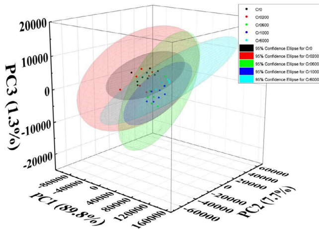
Fig. 12. 3D Score plot of Principal Components and their corresponding confidence (95%) ellipse based on different Cr 2 O 3 contents in UO 2 pellets. The total percent variance captured by each PC is shown in brackets along each axis. (For interpretation of the references to colour in this figure legend, the reader is referred to the web version of this article.)
