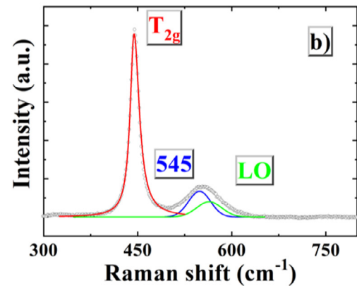
Fig. 15. Raman spectra of a UO 2 disk doped with a) 600 ppm and b) 1000 ppm of Cr 2 O 3 by Lorentzian peaks at 445, 545 and 570 cm -1 .
