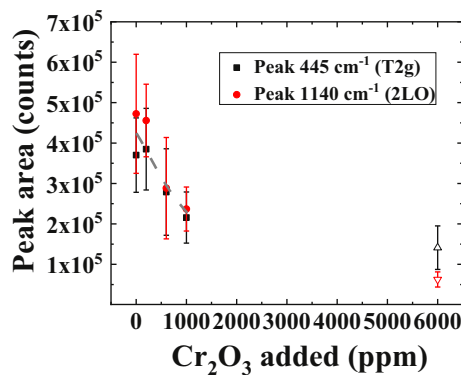
Fig. 14. Area evolution of the T 2g (445 cm -1 ) and 2LO (1140 cm -1 ) bands with Cr 2 O 3 concentration. Solid symbols correspond to samples with Cr 2 O 3 content lower than the solubility limit, while open triangles represent the pellet doped with 6000 ppm of Cr 2 O 3 , which is higher than the solubility limit. Dashed line represents a guide to the eye to show the general trend of data. Uncertainty bands correspond to the repeatability of the measurements.
