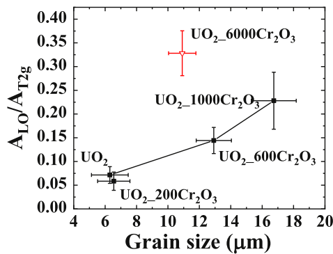
Fig. 17. LO band area ratio vs grain size of the analyzed pellets. Black squares correspond to samples with Cr 2 O 3 content lower than the solubility limit, while the open triangle represents the pellet doped with 6000 ppm of Cr 2 O 3 , which is higher than the solubility limit. Uncertainty bands correspond to the repeatability of the measurements.
