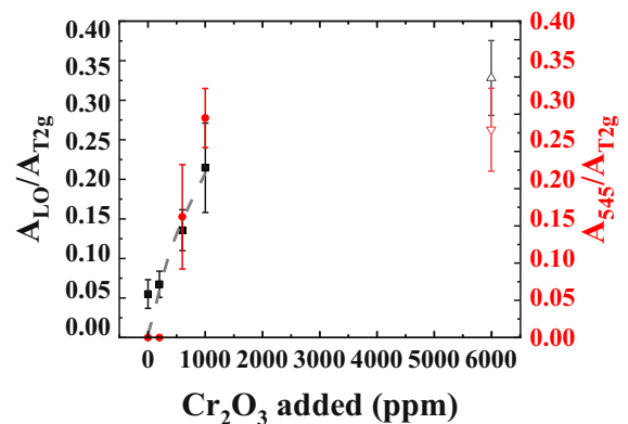
Fig. 16. Evolution of the intensity of the peaks at 570 cm -1 (LO band, black squares) and 545 cm -1 (red circles), both referred to the T 2g band, with the Cr 2 O 3 content. Solid symbols correspond to samples with Cr 2 O 3 content lower than the solubility limit, while open triangles represent the pellet doped with 6000 ppm of Cr 2 O 3 , which is higher than the solubility limit. Dashed line represents a guide to the eye to show the general trend of data. Uncertainty bands correspond to the repeatability of the measurements. (For interpretation of the references to colour in this figure legend, the reader is referred to the web version of this article.)
