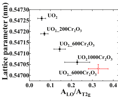
Fig. 18. Lattice parameter vs A_{LO}/A_{T2g} peaks ratio. Black squares correspond to samples with Cr 2 O 3 content lower than the solubility limit, while the open triangle represents the pellet doped with 6000 ppm of Cr 2 O 3 , which is higher than the solubility limit. Uncertainty bands correspond to the repeatability of the measurements.
