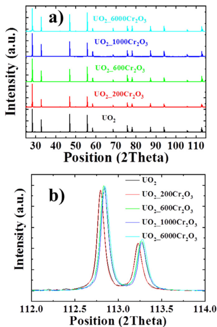
Fig. 7. a) Diffraction patterns of the studied samples and b) the (531) K\alpha_{1,2} doublet at 113^\circ of the normalized diffraction patterns.
