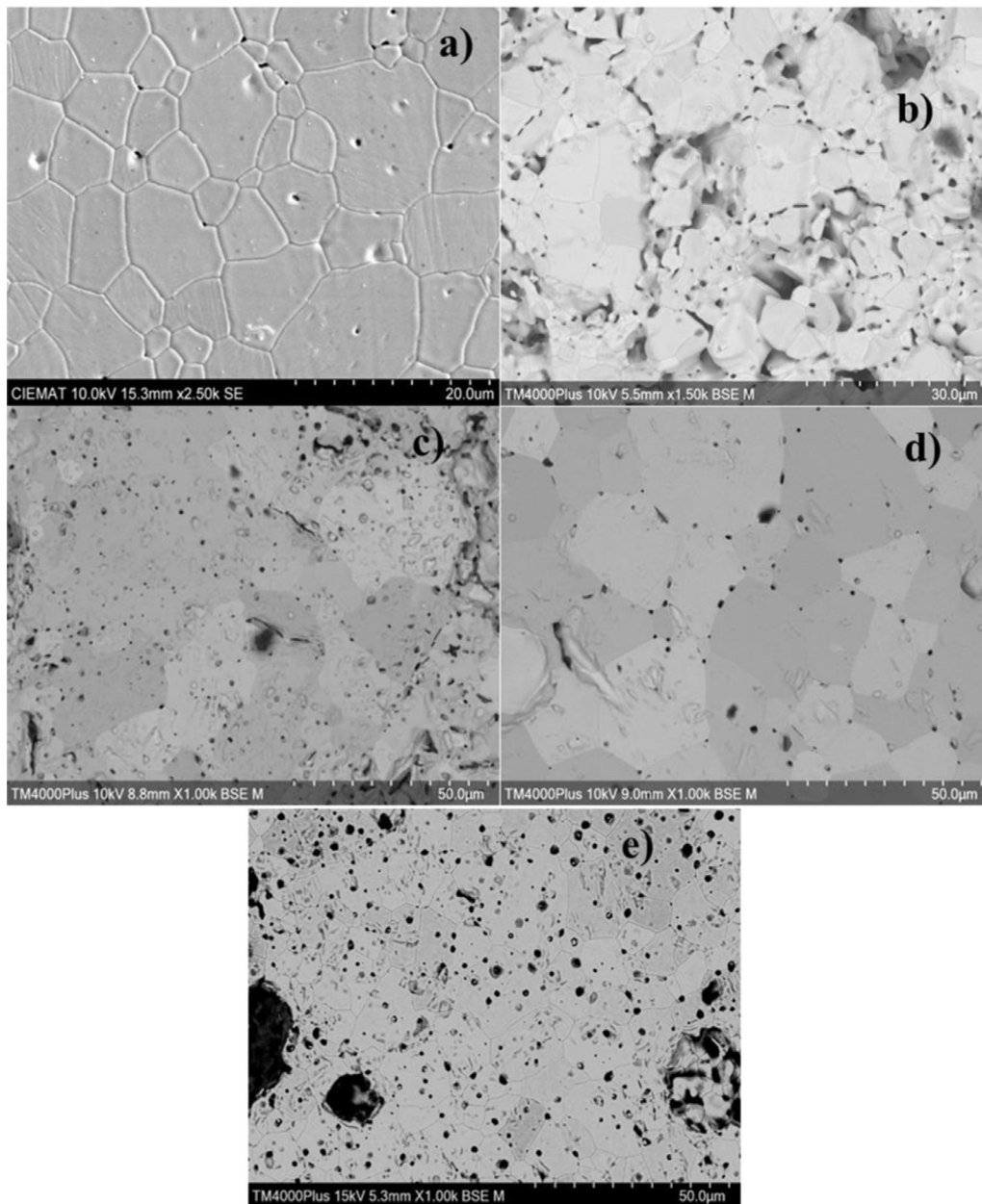
Fig. 4. Representative SEM images of the analyzed pellets: a) pure \text{UO}_2 , b) \text{UO}_2\text{-200Cr}_2\text{O}_3 , c) \text{UO}_2\text{-600Cr}_2\text{O}_3 , d) \text{UO}_2\text{-1000Cr}_2\text{O}_3 , e) \text{UO}_2\text{-6000Cr}_2\text{O}_3 .
